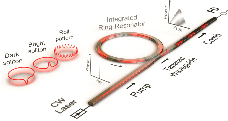
FIG. 1. Schematic representation of microcomb generation. A microresonator is pumped by a resonant single-frequency laser. A spatiotemporal pattern is created inside the cavity via the interplay between laser power, losses, nonlinearity, dispersion, and frequency detuning. This process outputs a train of optical pulses that yield an optical frequency comb in the spectral domain. We have depicted on the left some of the intracavity patterns that can be created, such as dark solitons, bright solitons, or roll patterns.
