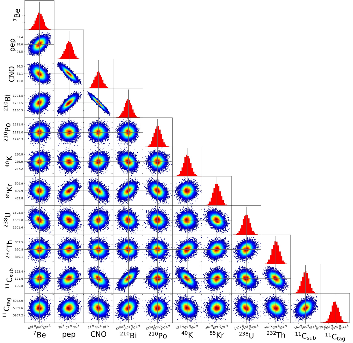
Figure 5. Example correlation plots obtained from the sensitivity study, performing 10^4 fits in the Medium Background scenario for six years of data taking. The red histograms display the distributions of the best-fit reconstructed rates, expressed in cpd/kton units. The non-diagonal frames report the correlation plots among the different species: the rates density increases going from blue to red tones.
