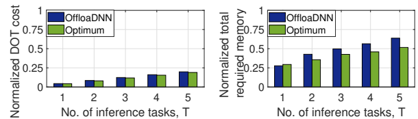
Fig. 7. Small-scale scenario: Comparison of the total DOT cost and memory utilization due to active DNN blocks, under the optimal and the OffloadDNN strategies, as the number of inference tasks T varies.
