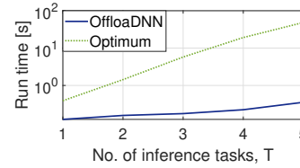
Fig. 6. Comparison of the average runtime taken by the optimum and the OffloadDNN solution strategies, in the small-scale scenario, as the number of inference tasks T varies.
