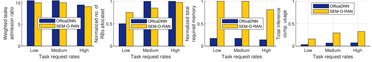
Fig. 10. Large-scale scenario: OffloadDNN vs SEM-O-RAN as the tasks rate varies: (left) average task admission ratio weighted by task priority; (center-left) total no. of allocated RBs, normalized to the maximum available; (center-right) total memory utilization; (right) total compute usage for the admitted tasks, normalized to the maximum available.
