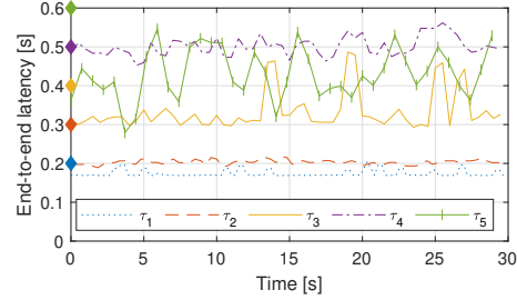
Fig. 11. Experiments in Colosseum: time evolution of task end-to-end latency and maximum latency targets (diamond markers). For clarity, a moving average with a window size of 3 samples is used.
