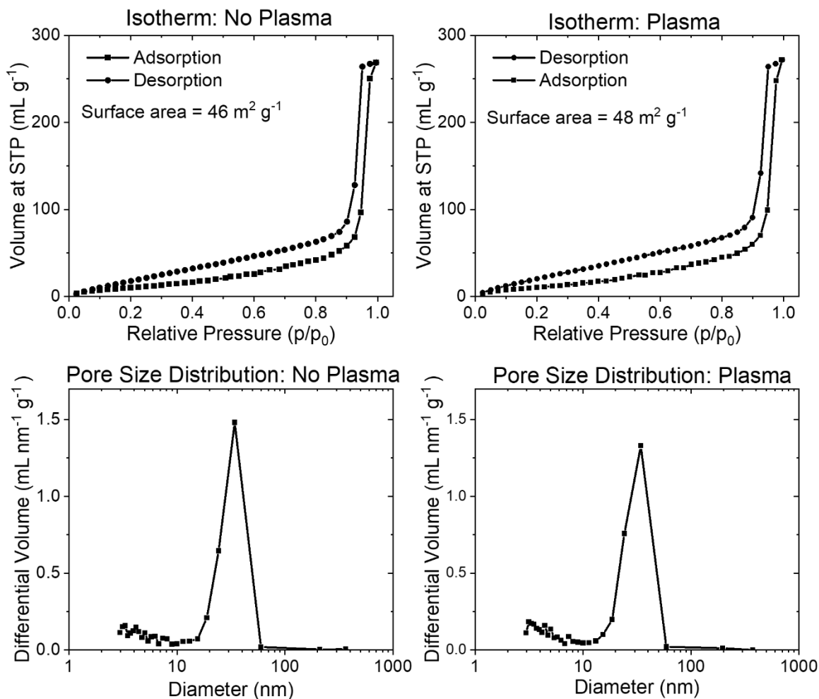
Figure 7. Type IV Isotherms and corresponding pore size distributions from nitrogen adsorption analysis of PCOE membranes derived from LCL [25-51-25] before and after plasma etching. Surface area is determined using the BET equation and pore size distribution is determined using the BJH method. Mode pore diameters are calculated to be 34 nm in both samples.
