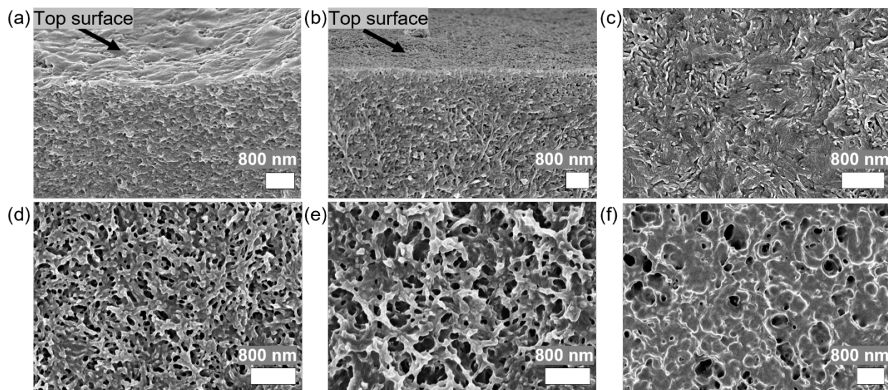
Figure 6: (a–b) SEM images of cryo-fractured nanoporous PCOE membranes taken near the surface of membranes derived from LCL [25-51-25]. Both samples were solvent cast followed by annealing for 20 minutes at 70 °C prior to PLA etching. Additionally, sample (b) was plasma etching for 60 seconds following PLA etching. (c–f) Surface SEM images of membranes plasma-etched for (c) 0 seconds, (d) 60 seconds, (e) 120 seconds, and (f) 600 seconds.
