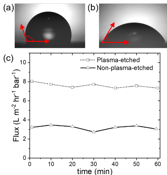
Figure 8. Water contact angle measurements of (a) non-plasma-etched and (b) plasma-etched NPMs derived from LCL [25-51-25], and (c) representative water flux measurement.
