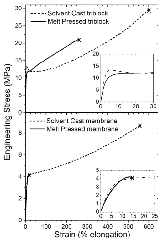
Figure 5. Representative stress–strain curves from uniaxial tensile testing of LCL [25-51-25] triblock films (top) and nanoporous membranes (bottom) prepared by different processing methods. Insets: low-strain regions enlarged for clarity.
