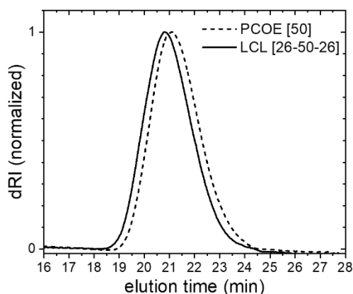
Figure 1. Representative SEC and of PCOE homopolymer and LCL triblock copolymer.
