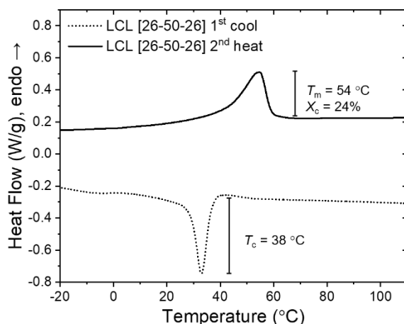
Figure 2. DSC of LCL triblock copolymer after precipitation with a heating/cooling rate of 10 °C min -1 . Traces represent the first cool and second heat.
