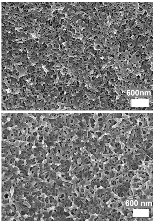
Figure 4. Cross-sectional SEM images of cryo-fractured nanoporous PCOE membrane derived from (top) LCL [26-50-26] and (bottom) [49-95-49]. Samples coated with 2 nm platinum.
