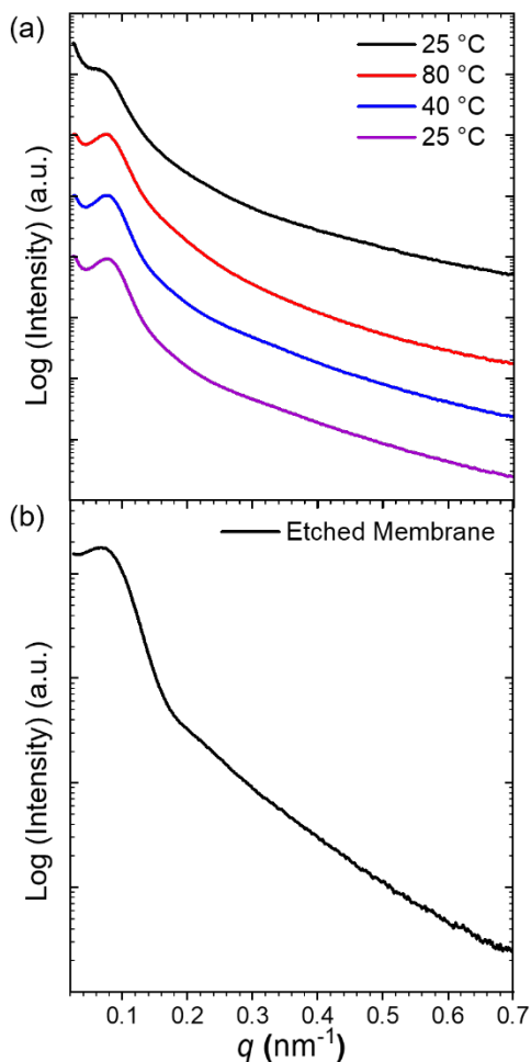
Figure 3. (a) Variable temperature SAXS analysis of solvent cast LCL [26-55-26] triblock copolymer films. Curves correspond to 25 °C (black) as cast, 80 °C (red), 40 °C (blue), and 25 °C (purple) after thermal treatment. Samples were held isothermally at 80 °C for 20 minutes and 40 °C for 30 minutes. Shifted vertically for clarity. (b) Room temperature SAXS analysis of nanoporous PCOE derived from LCL [28-49-28].
