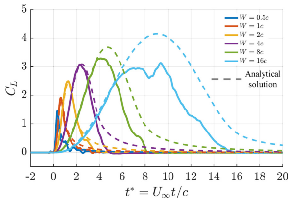
FIG. 16. Computational and theoretical lift transients for a sine-squared gusts, varying the gust width at a gust ratio of 0.8 [64].
