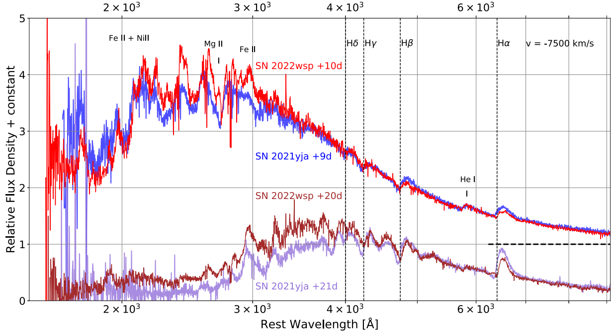
Figure 1. HST/STIS UV-optical spectra of SN 2022wsp at +10 and +20 days compared with those of SN 201yja at similar phases. All spectra have been dereddened. The SN 2022wsp flux density has been scaled by the same constant for both days such that the continuum level redward of 7000 Å matches that of SN 201yja, demonstrating the dramatic evolution and variation in the UV, while showing general agreement at optical wavelengths. The spectra have also been shifted arbitrarily by a constant for easier comparison. The wavelength scale has been corrected to the rest frame using the recession velocity of the host galaxy. Balmer lines at an expansion velocity of v = 7500 \text{ km s}^{-1} are marked by vertical dotted lines. The zero flux level of the top two spectra is indicated by the horizontal dashed line.
