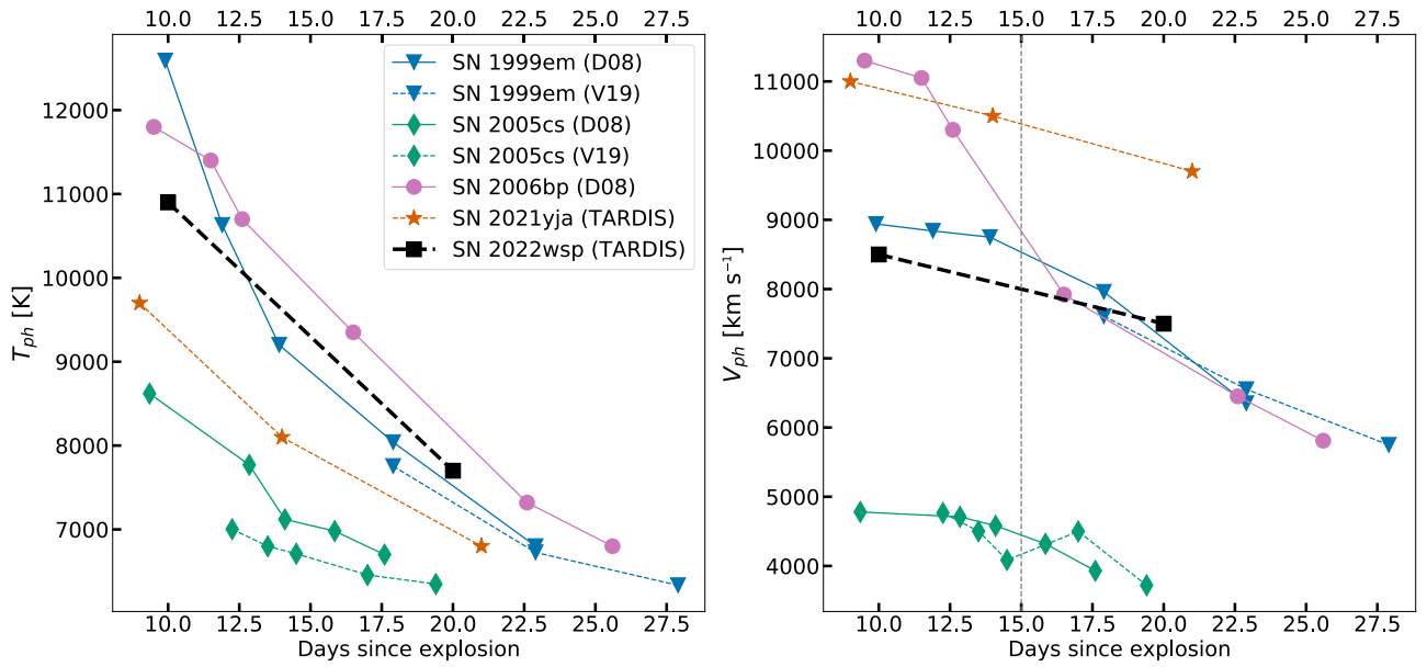
Figure 4. Temporal evolution of the photospheric temperature T_{ph} (left) and photospheric velocity v_{ph} (right) of SN 2022wsp obtained from the TARDIS fit to its days +10 ( T_{ph}=10,900 K, v_{ph}=8500 km s -1 ) and +20 ( T_{ph}=7700 K, v_{ph}=7500 km s -1 ) spectra compared to those of SNe 1999em, 2005cs, 2006bp, and 2021yja (Dessart et al. 2008, D08; Vogt et al. 2019, V19; Vasylyev et al. 2022). Vertical dashed line indicates the velocity at days +15, v_{d15} , for comparison purposes.
