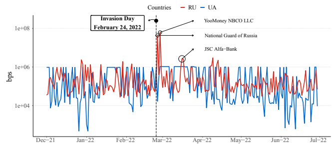
Fig. 2. A time series of DDoS rates (bps) for both Russia and Ukraine during the 7-month analysis period.
