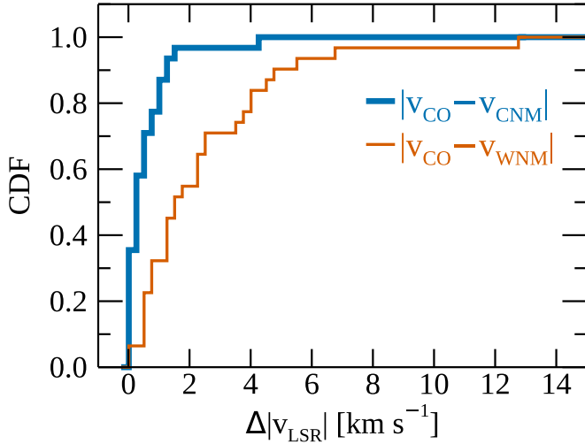
Figure 5. CDF of the absolute velocity difference between H I and CO (CNM and CO in thick blue; WNM and CO in thin tan). For these CDFs, H I components that are closest to the observed CO emission in velocity were considered.
