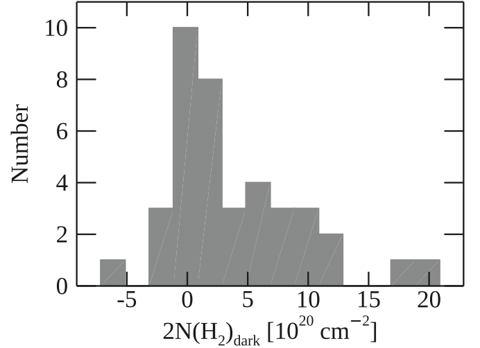
Figure 4. Histogram of the CO-dark H 2 column density for the 39 CO non-detected LOSs.
