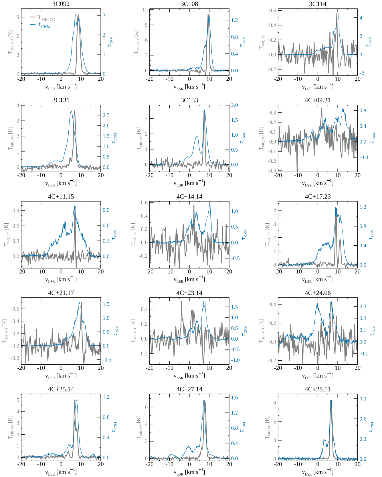
Figure A1. Comparison between the H I absorption (thin blue) and CO emission (thick gray) spectra toward the 19 CO-detected LOSs. The spectra are aligned at peaks for ease of comparison.
