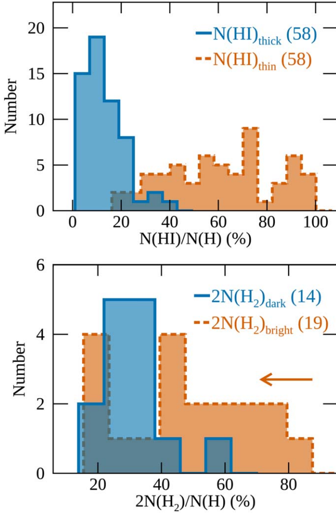
Figure 3. Fraction of each gas phase with respect to the total hydrogen. (Top) Optically thick and thin H I in solid blue and dashed tan. (Bottom) CO-dark and CO-bright H 2 in solid blue and dashed tan. The leftward arrow indicates that the derived fractions for CO-bright H 2 are upper limits.
