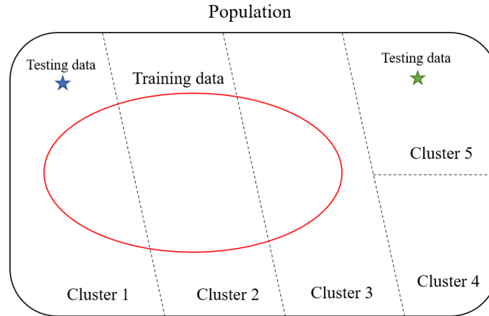
Figure 1: An illustration of unseen-cluster problem
