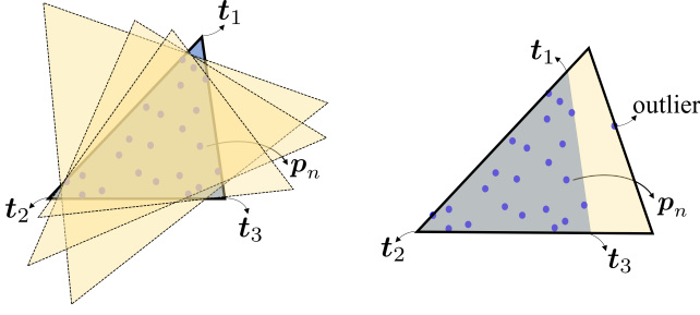
Fig. 1. Illustrating the effect of outlier data points in volume minimization. The dots denote the vectors \mathbf{p}_n . Blue shaded region denote the ground-truth \text{conv}(\mathbf{t}_1, \dots, \mathbf{t}_K) . Left) The minimum volume simplex (outlined by the black bold line) is same as \text{conv}(\mathbf{t}_1, \dots, \mathbf{t}_K) . Right) An outlier impacts volume minimization. Here the minimum volume simplex is different from \text{conv}(\mathbf{t}_1, \dots, \mathbf{t}_K) .
