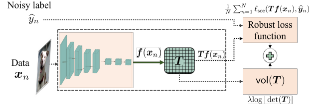
Fig. 2. The proposed RobVolMinNet framework.
