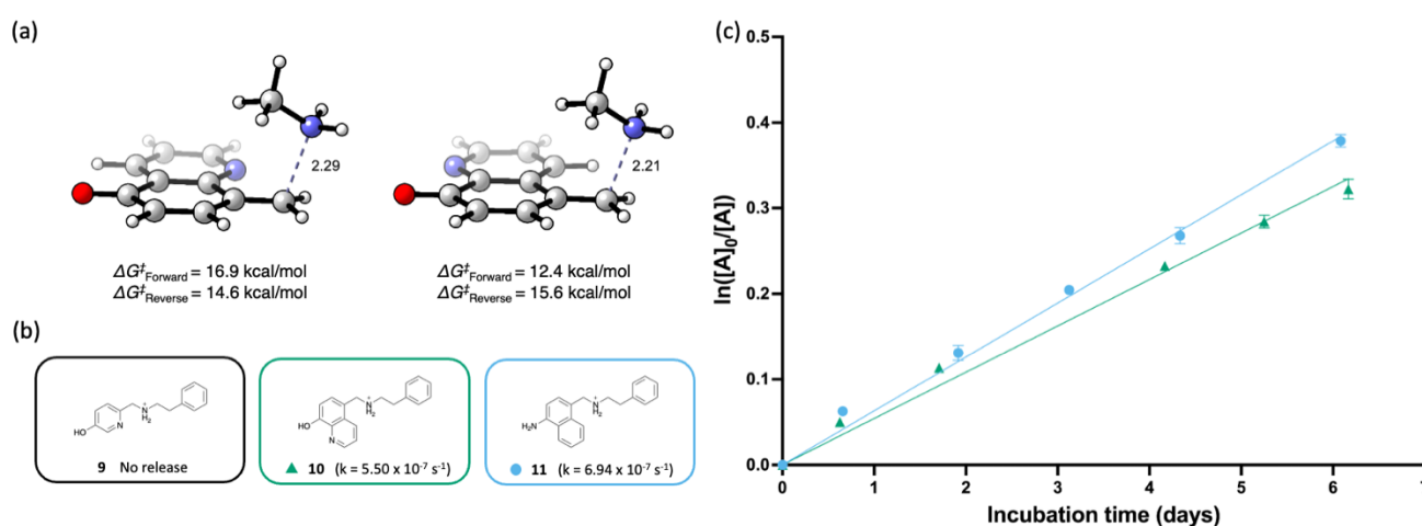
Figure 4. (a) TS1 structures calculated at the B3LYP-D3/6-31+G(d,p), CPCM(water) level of theory for 5- and 8-hydroxyquinoline benzylammoniums and calculated free energies of activation for the forward and reverse reactions at the M06-2X/aug-cc-pVTZ, CPCM(Water)//B3LYP-D3/6-31+G(d,p), CPCM(Water) level of theory. (b) Library of pyridine-, quinoline-, and azanaphthalene-based phenethylamine conjugates synthesized and their experimentally determined release rate constants. (c) First-order plot of phenethylamine release kinetics ( n = 3 , some error bars are smaller than markers) carried out at 5 mM of the hydroxy- or azabenzyllammonium in a 1:1 mixture of methanol and 0.1 M Tris buffer (pH 7.4).
