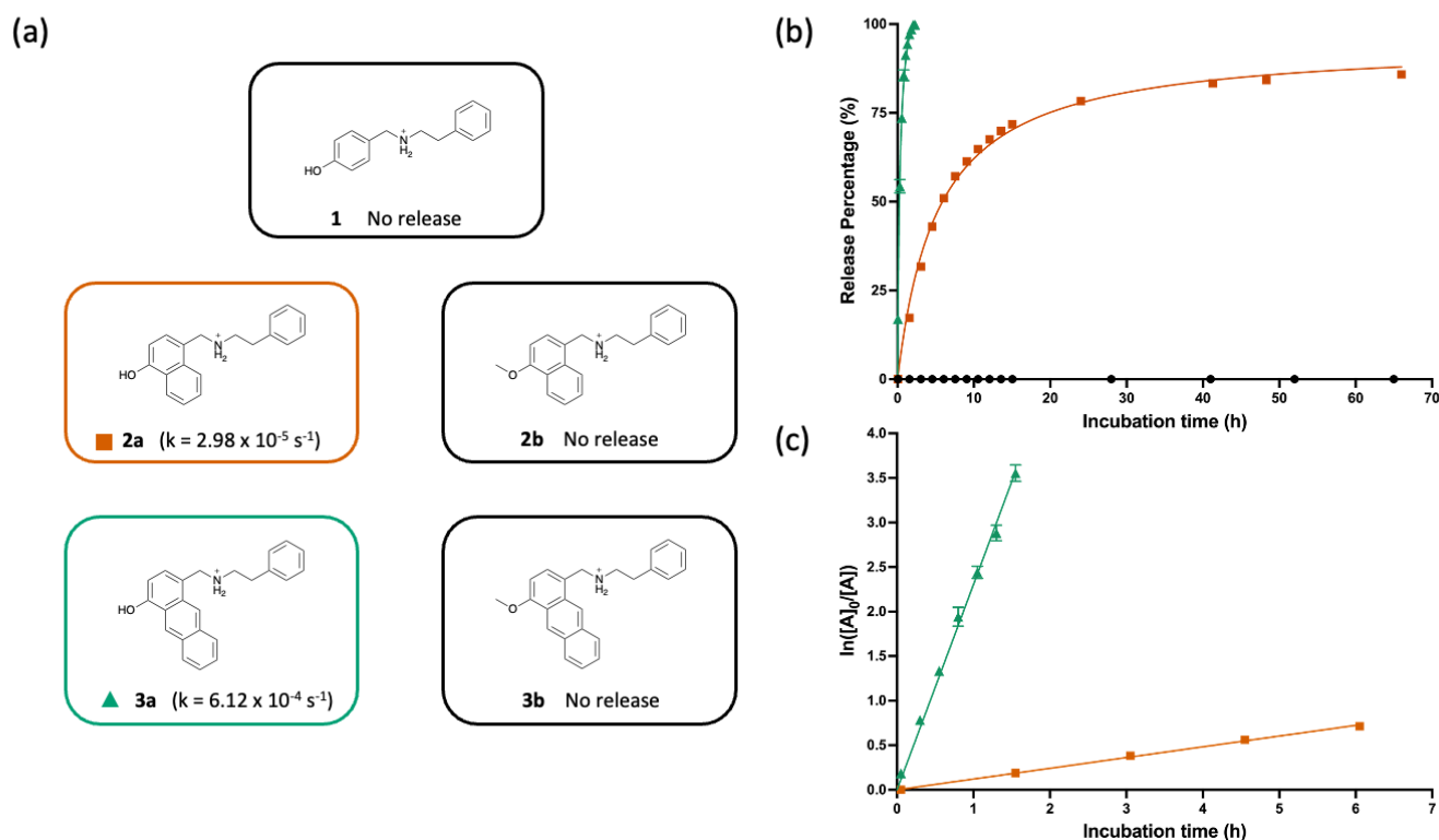
Figure 3. (a) Library of polycyclic aromatic – phenethylamine conjugates prepared and their experimentally determined release rate constants. (b) Phenethylamine release kinetics of 1 , 2a , and 3a ( n = 3 , some error bars are smaller than markers) carried out at 5 mM of the benzene- or naphthalene-hydroxybenzylammoniums or 1 mM of the anthracene-hydroxybenzylammonium in a 1:1 mixture of methanol and 0.1 M Tris buffer (pH 7.4). (c) First-order plot of phenethylamine release kinetics of 2a and 3a ( n = 3 , some error bars are smaller than markers).
