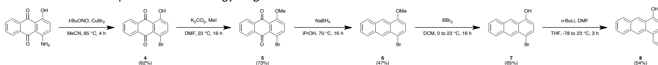
Scheme 1. Synthesis of 1,4-anthracene hydroxybenzaldehyde 8 .
