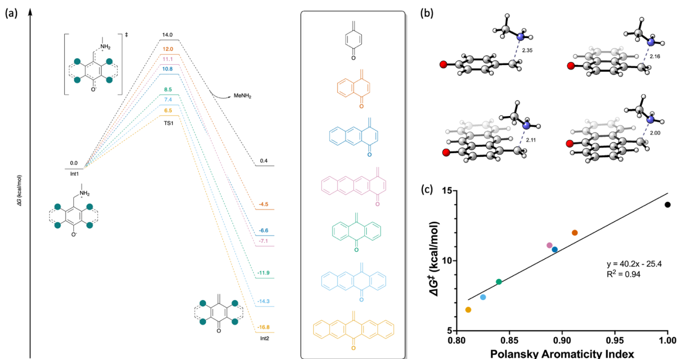
Figure 2. (a) Free energy diagrams for polycyclic aromatic hydroxybenzylammonium release calculated at the M06-2X/aug-cc-pVTZ, CPCM(Water)//B3LYP-D3/6-31+G(d,p), CPCM(Water) level of theory. (b) TS1 geometries calculated for 1,4-benzene, 1,4-naphthalene, 1,4-anthracene, and 9,10-anthracene-based hydroxybenzylammoniums. (c) Calculated free energy of activation at the aforementioned level of theory plotted against the corresponding Polansky Aromaticity Index of the parent hydrocarbon scaffold.
