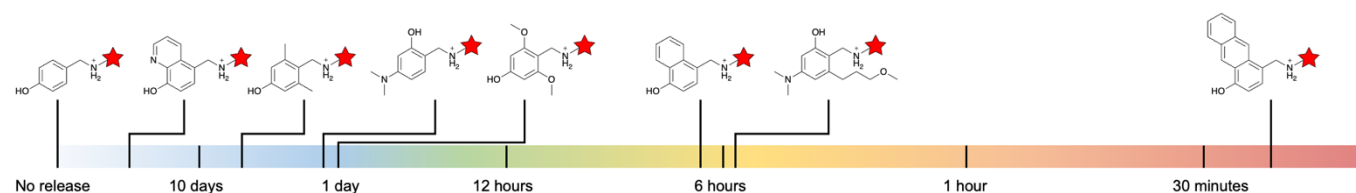
Figure 5. Release half-life spectrum of hydroxybenzylammonium molecules. Release half-lives displayed are from this report as well as our previous article. 26
