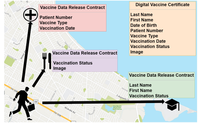
Figure 1: An essential function of SecureCheck: data owners leverage contracts to release specific data for various locations, e.g., hospitals, restaurants, and schools.
