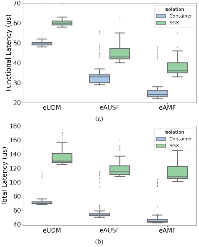
Fig. 9: (a) Functional ( L_F ) and (b) Total ( L_T ) latency of the P-AKA modules
