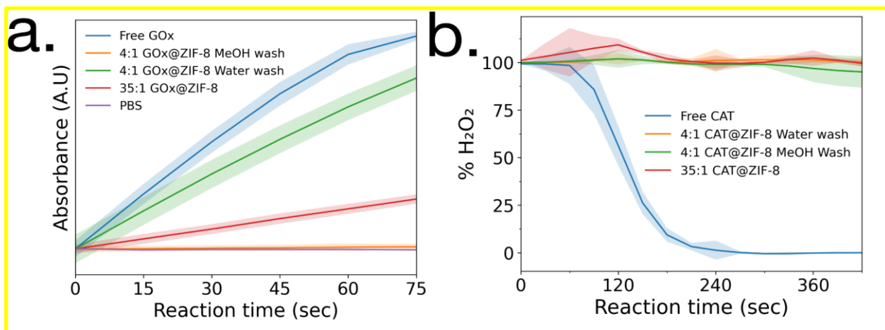
Figure 2: Enzyme activity assays of (a.) GOx@ZIF-8 and (b.) CAT@ZIF-8 at a variety of synthetic conditions. Standard deviations are shown as highlighted sections.
