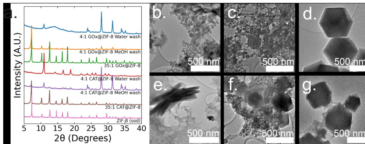
Figure 1. (a.) P-XRD patterns of CAT@MOFs and GOx@MOFs at 4:1 HmIM:Zn ratios with either water or methanol washes and at 35:1 HmIM:Zn. Dry-state TEM images of (b.) 4:1 GOx@ZIF-8 with 3x water washes showing amorphous aggregates and sheets, (c.) 4:1 GOx@ZIF-8 with 3x methanol washes showing both rhombic dodecahedra and amorphous morphologies, (d.) 35:1 GOx@ZIF-8 showing a rhombic dodecahedron morphology, (e.) 4:1 CAT@ZIF-8 with 3x water only washes showing amorphous aggregates and sheets, (f.) 4:1 CAT@ZIF-8 with 3x methanol washes showing a mixture of rhombic dodecahedra, sheets and amorphous morphologies, (g.) 35:1 CAT@ZIF-8 showing rhombic dodecahedra and amorphous morphologies.
