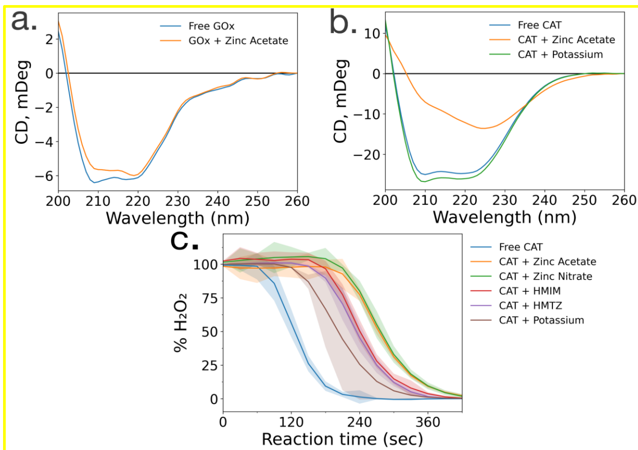
Figure 3: Circular dichroism spectra of (a.) glucose oxidase in the absence (blue) and presence (orange) of zinc acetate and (b.) catalase in the absence (blue) and presence of zinc acetate (orange) and potassium acetate (green). (c.) Catalase activity in the presence of MOF precursors and various ions, where standard deviations are shown as highlighted sections.
