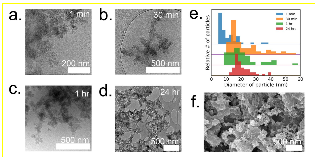
Figure 4: Time resolved cryoTEM of 4:1 GOx@ZIF-8 at (a.) 1 min, (b.) 30 min, and (c.) 1 hr. (d.) Dry-state TEM of 4:1 GOx@ZIF-8 after washes with water. (e.) Particle size analysis at 1 min (blue), 30 min (orange), 1 hr (green), and 24 hrs (red). (f.) SEM of 4:1 GOx@ZIF-8 after washes with water.
