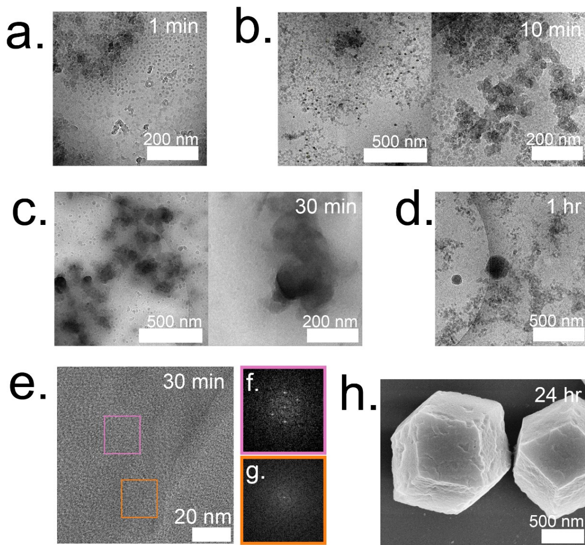
Figure 5: Time resolved cryoTEM of 35:1 GOx@ZIF-8 at (a.) 1 min, (b.) 10 min, (c.) 30 min and (d.) 1 hr. (e.) Lattice resolution cryoTEM image of 35:1 and corresponding selective area fourier transform of (f.) pink region and (g.) orange region from image. (h.) SEM of 35:1 GOx@ZIF-8 after water washes.
