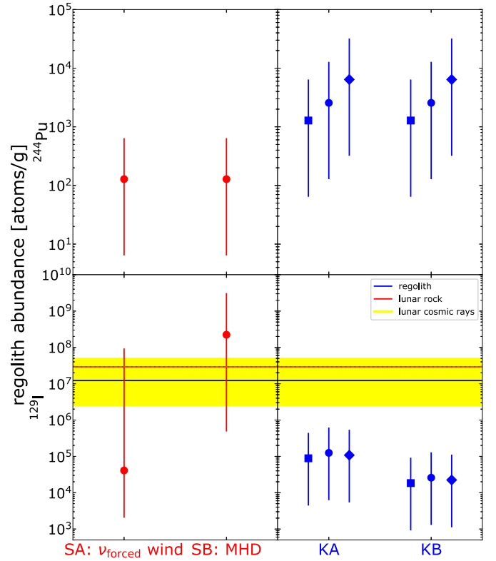
Fig. 2. Lunar abundances of ^{244}\text{Pu} and ^{129}\text{I} , for supernova (left) and kilonova (right) models. Supernova models are for an event at 3 Myr ago with flux spread over 1 Myr; left points are for a forced neutrino wind and right points are for a magnetohydrodynamic supernova. Kilonova models are for events 10, 20, and 50 Myr ago. The vertical bars include estimates of the nuclear uncertainties influencing the abundance predictions, as described in [57]. The cosmic-ray background (shown in yellow) is proportional to the abundance of barium in the regolith; the band shown is for a barium mass fraction X_{\text{Ba}} = 42 - 850 ppm. The regolith and rock results shown are for sources with high X_{\text{Ba}} . We see that the supernova signal is above background, while the kilonova signals are not, unless X_{\text{Ba}} is small. A regolith measurement of ^{129}\text{I} in conjunction with barium could distinguish between these cases.
