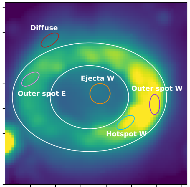
Figure 10. Small regions (in colour) used for SEDs in Fig. 11 and the white elliptical annulus used for the ring and outer spots photometry in Fig. 12 (also in Appendix B), overlaid on F323N image.
