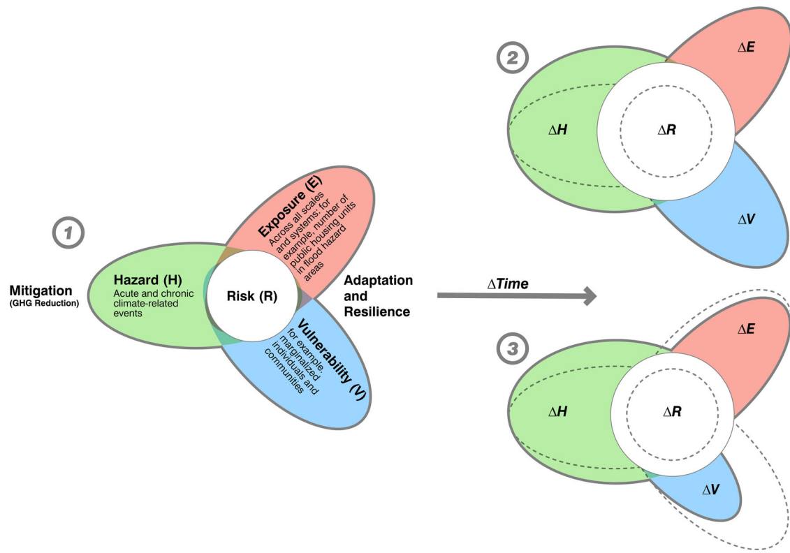
FIGURE 1 The impact of the dynamic components of climate risk (R) on its temporal evolution. Graphic 1 shows the baseline condition. Graphic 2 shows the impact of sluggish climate mitigation on the magnitude of the hazard (H) and the subsequent increase in climate risk. Graphic 3 shows that even with the implementation of climate adaptation and resilience strategies that reduce vulnerability (V) and exposure (E), climate risk may increase if the magnitude of the hazard continues to increase (adapted from Ref. 1).
