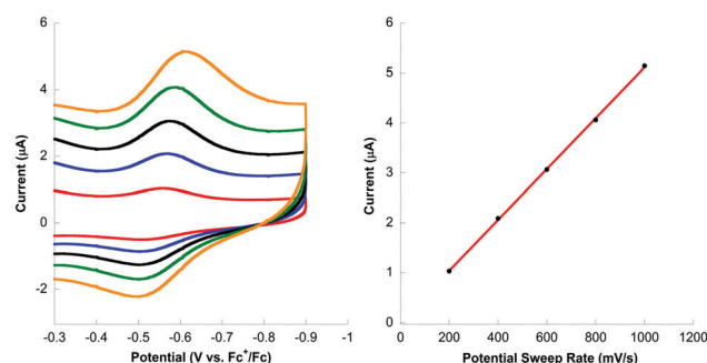
Fig. 3 Left: Cyclic voltammograms of 2 adsorbed to the surface of a glassy carbon electrode in 5 mL of 0.1 M TBAPF 6 in \text{CH}_3\text{CN} taken at scan rates of 200 (red), 400 (blue), 600 (black), 800 (green), and 1000 (orange) \text{mV s}^{-1} . Right: Cathodic peak current versus potential sweep rate for 2 ( R^2 = 0.99972 ).
