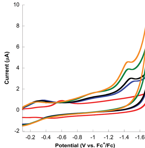
Fig. 5 Cyclic voltammograms of surface adsorbed 2 in 5 mL of 0.1 M TBAPF 6 in CH 3 CN in the presence of no acid (red), 0.4 mM (blue), 0.8 mM (black), 1.2 mM (green), and 1.6 mM (orange) at 200 mV s -1 .
