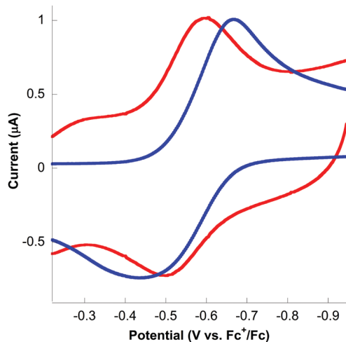
Fig. 4 Cyclic voltammograms of 2 (red) adsorbed to the surface of a glassy carbon electrode and 0.1 mg of 1 (blue) in 5 mL of 0.1 M TBAPF 6 in CH 3 CN taken at 200 mV s -1 .
