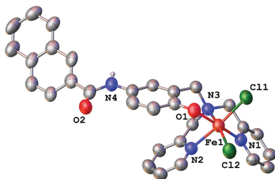
Fig. 2 ORTEP diagram of 2 with Fe (orange), O (red), N (blue), Cl (green), and C (gray). Hydrogen atoms are omitted for clarity.
