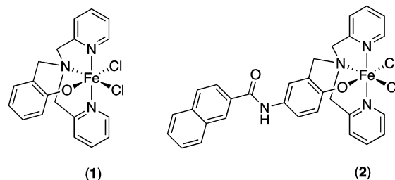
Fig. 1 Left: Iron polypyridyl monophenolate parent catalyst ( 1 ). Right: Naphthalene-terminated iron polypyridyl monophenolate parent catalyst ( 2 ).
