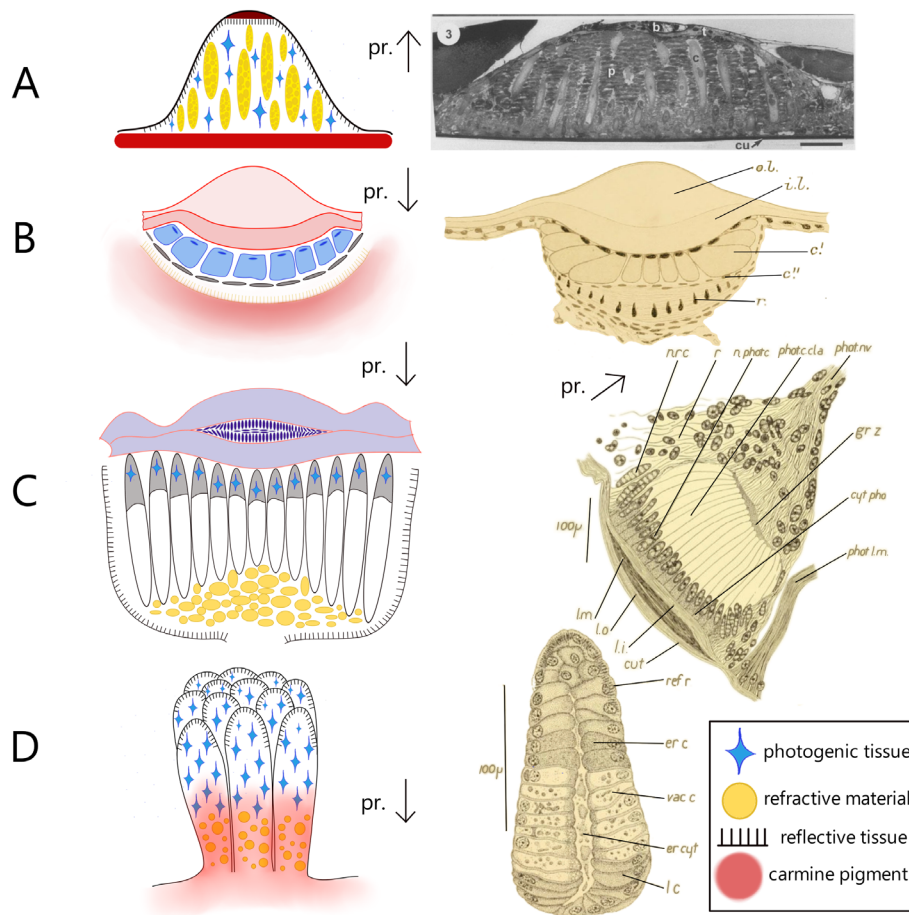
Fig. 2. Diversity of photophore structure in decapod shrimps. (A) Diagram of an unlensed photophore of a sergestid shrimp (left) and histology from Nowel et al. (2002) (right). b , blood vessel; c , columnar cells; cu , cuticle; p , darkly staining material in photogenic cells; t , thin tapetal layer. (B) Diagram of lensed photophore of a sergestid shrimp (left) and schematic from Kemp (1910a) (right). c' , first cellular layer; c'' , second cellular layer; i.l. , inner layer of lens; o.l. , outer layer of lens; r. , reflector or striated layer. (C) Diagram of pigmented lensed photophore of oplophorid pleopod (purple shading indicates pigmented lens derived from cuticle; grey shading in columnar cells indicates portion of cell with photogenic material) (left) and histological schematic from Dennell (1940) (right). cut , cuticle; cyt pha , cytoplasm of photogenic cell; gr z , granular zone; l.i. , inner layer of lens; lm , middle layer of lens; l.o. , outer layer of lens; phot c cla , clear area of photogenic cell; phot.l.m. , longitudinal muscle of photophore; phot.nv , photophore nerve; n phot c , nucleus of photogenic cell; nrc , nucleus of reflector layer; r , reflector. (D) Diagram of a cross section through a lobe of the organs of Pesta of Sergestidae (left) and a histological schematic of one of several tubules comprising each lobe of the organs of Pesta from Dennell (1940) (right). er c , erupting cell of tubule; er cyt , erupted cytoplasm lying within lumen of tubule; l c , 'lens' cell; ref r , refractile rods; vac c , vacuolated cell. The adjacent to each image depicts the direction of proximity towards the body (pr). In all cases, emitted light is in the opposite direction to the arrow.
