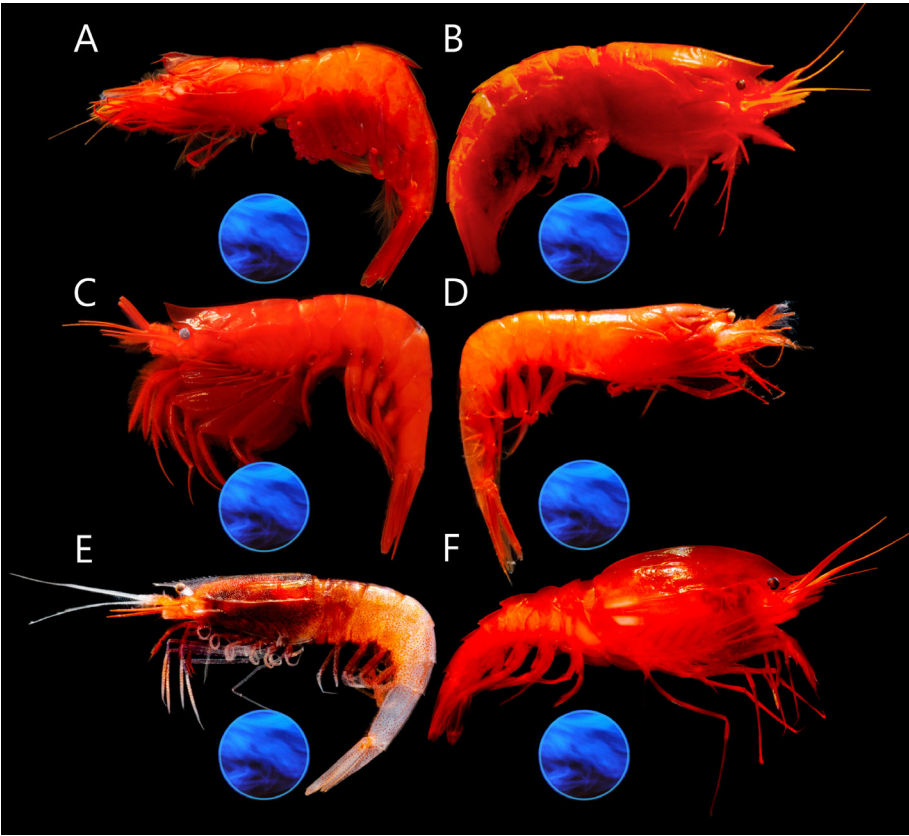
Fig. 7. (A) Acanthephyra stylostratis . (B) Acanthephyra sp. (C) Ephyra benedicti . (D) Hymenodora gracilis . (E) Meningodora vesca . (F) Notostomus gibbosus . All species produce bioluminescent secretions, as indicated by the blue circles. Photograph credits: D. Fenolio.
