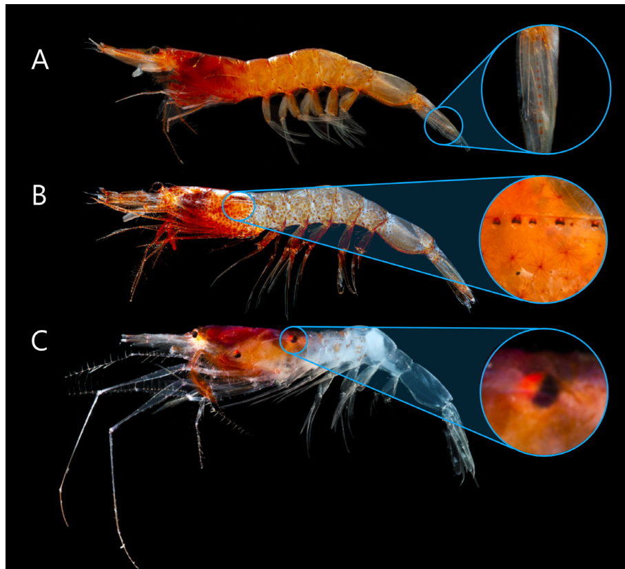
Fig. 4. (A) Gardinerosergia splendens , enlarged portion showing unlensed photophores of the uropod. (B) Challengerosergia hansjacobii , enlarged portion showing lensed photophores of the lateral carapace. (C) Allosergestes pectinatus , enlarged portion showing posterior lobe of organs of Pesta. Photograph credits: D. Fenolio.
