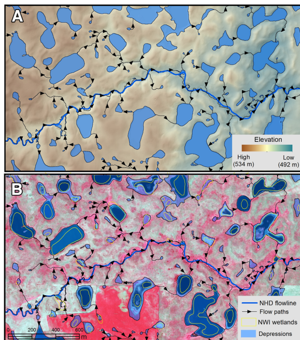
Figure 6. A and B Widespread spatial heterogeneity and climatic, volumetric, and geophysical characteristics control non-floodplain wetland biogeochemical (and hydrological) functions affecting watershed resilience. Wu and Lane (2017) A identified potential wetland depressions and connectivity flow paths to a National Hydrography Dataset (NHD) river in a North American watershed (Pipestem River, North Dakota, USA) using lidar; the variability in wetland size, estimated volume, perimeter to area (Cohen and others 2016) and bathymetric properties (Cheng and Basu 2017) were found by Evenson and others (2018) to affect biogeochemical and hydrological functions. In addition, Wu and Lane (2017) B contrasted lidar-based non-floodplain wetland depressions with the best available National Wetland Inventory (NWI) data, demonstrating both regional wetland expansion since the baseline aerial imagery were acquired, as well as limitations to remotely identifying non-floodplain wetland systems.
