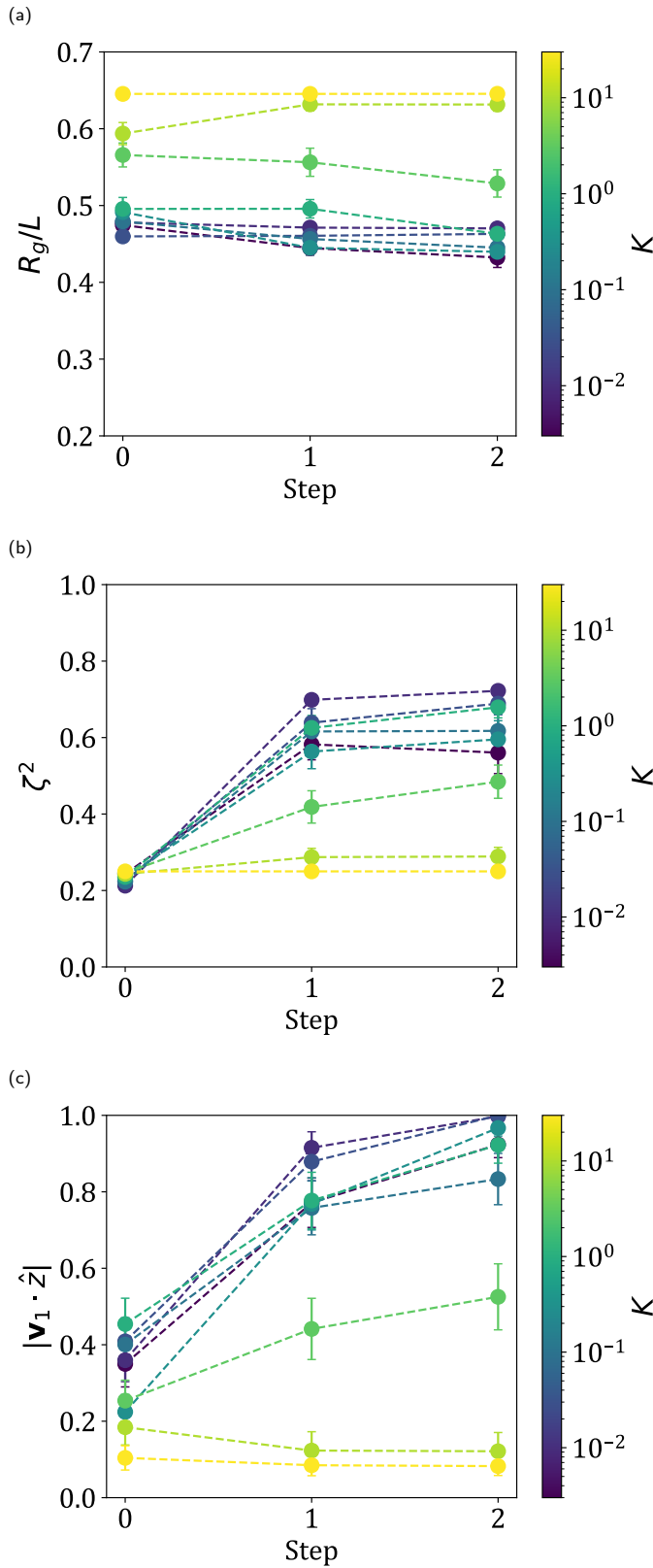
Fig. 8 Sheet (a) radius of gyration, (b) relative shape anisotropy, and (c) alignment averaged over the last 500 \tau of each step for Protocol 2. Error bars indicate 95% confidence intervals and dotted lines are drawn to guide the eye.
