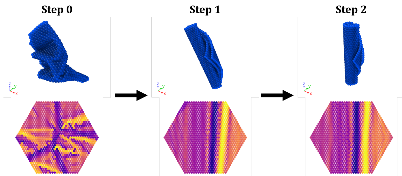
Fig. 7 Sample configurations (top) and their corresponding signed local mean curvatures (bottom), shown at the end of each constant \chi^{-1} step for Protocol 2. In configurations, x is the flow direction and y is the shear direction. Signed local mean curvature plots are all drawn to the same scale.
