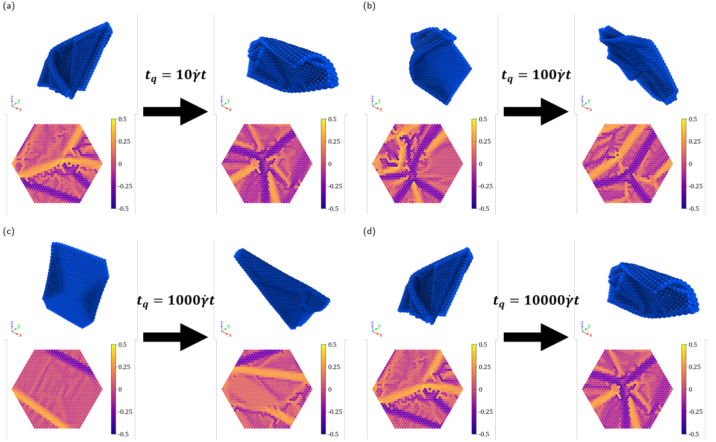
Fig. 3 Sample configurations (top) and their corresponding signed local mean curvatures (bottom), shown before (left) and after (right) annealing, for K = 0.03 and (a) t_q = 10\dot{\gamma}t , (b) t_q = 100\dot{\gamma}t , (c) t_q = 1000\dot{\gamma}t , and (d) t_q = 10000\dot{\gamma}t . Before annealing, sheets are sheared with a constant \chi^{-1} = 4.1 \times 10^2 , which is in the tumbling regime. In configurations, x is the flow direction and y is the shear direction. Signed local mean curvature plots are all drawn to the same scale.
