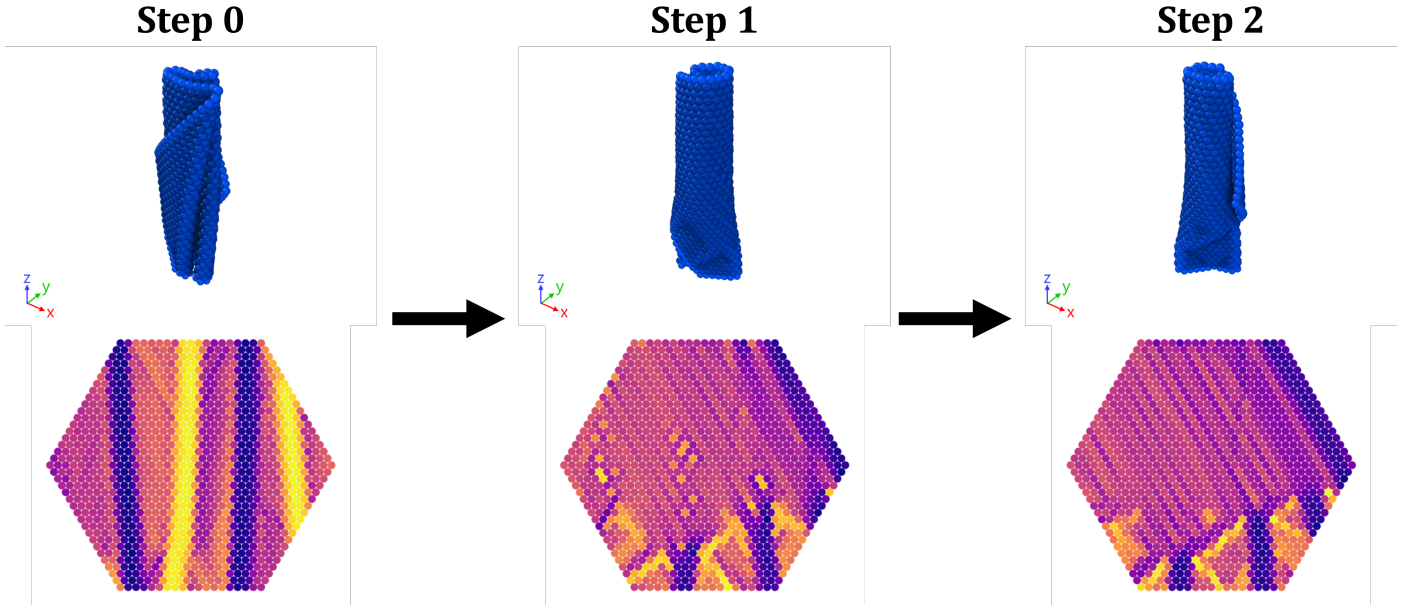
Fig. 5 Sample configurations (top) and their corresponding signed local mean curvatures (bottom), shown at the end of each constant \chi^{-1} step for Protocol 1. In configurations, x is the flow direction and y is the shear direction. Signed local mean curvature plots are all drawn to the same scale.
