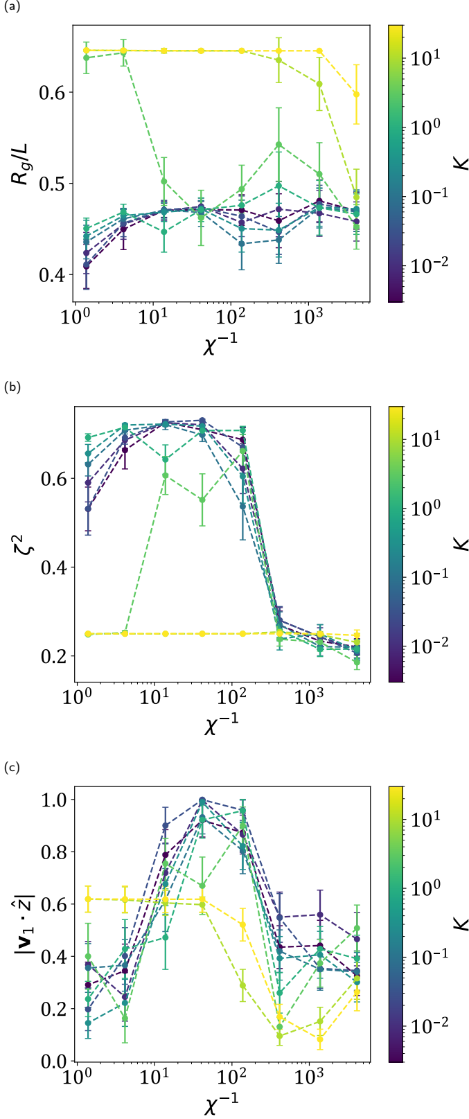
Fig. 1 (a) Radius of gyration, (b) relative shape anisotropy, and (c) alignment (from the minimum bounding ellipsoid) starting from flat initial configurations and averaged over the last 200\dot{\gamma}t and all \phi . Error bars are 95% confidence intervals. Dotted lines drawn to guide the eye. Recreated from previous work 1
