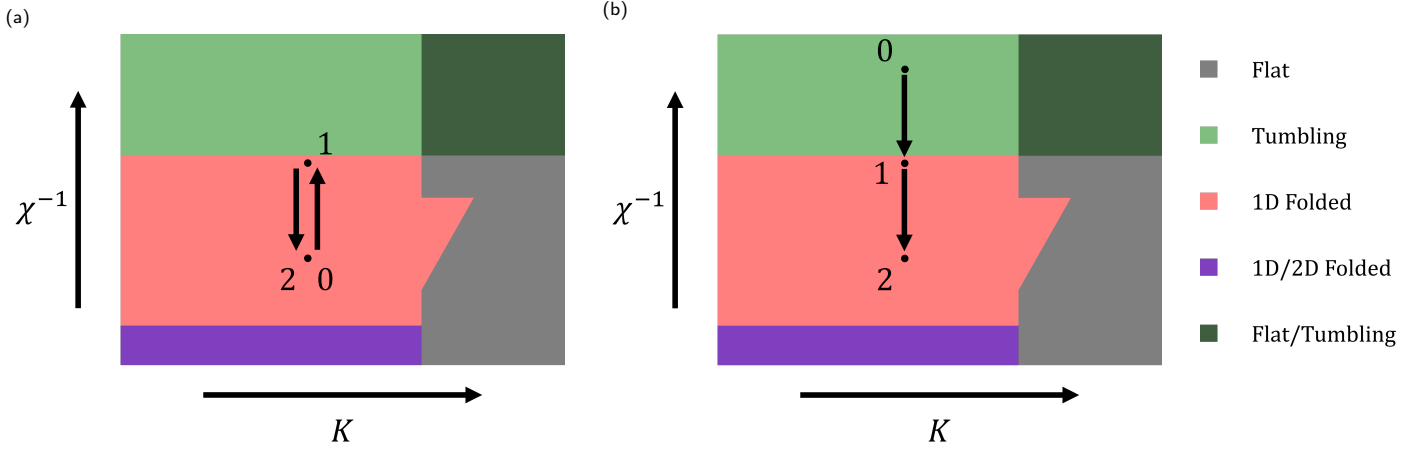
Fig. 2 Abstractions of different annealing protocols. Shaded regions denote the steady state conformational phase map discovered in our prior study 1 . Dots with numbers indicate constant \chi^{-1} simulations run for 2000\dot{\gamma}t . Arrows represent a factor of 10 change in \chi^{-1} . (a) Protocol 1, which starts at \chi^{-1} = 1.4 \times 10^1 . (b) Protocol 2, which starts at \chi^{-1} = 1.4 \times 10^3 .
