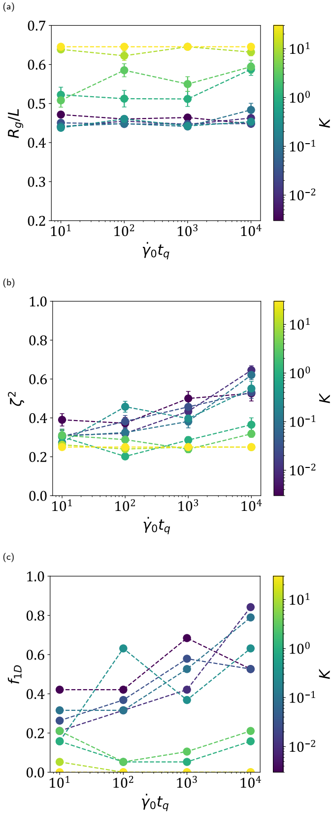
Fig. 4 Sheet (a) radius of gyration and (b) relative shape anisotropy as a function of quench time, averaged over the last 500\dot{\gamma}_0 t of the no shear portion of annealing simulations and all \phi . Error bars indicate 95% confidence intervals and dotted lines are drawn to guide the eye. (c) The fraction of sheets which were 1D folded after annealing.
