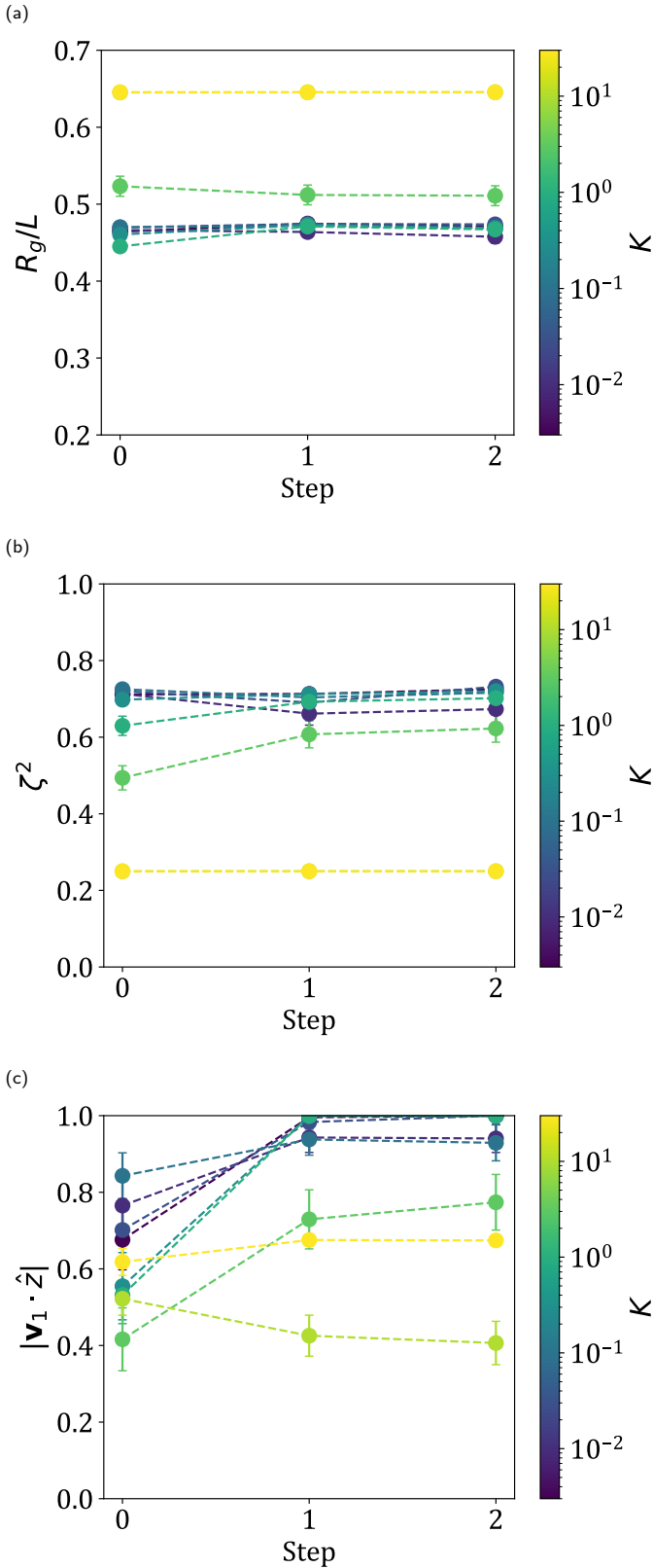
Fig. 6 Sheet (a) radius of gyration, (b) relative shape anisotropy, and (c) alignment averaged over the last 500\gamma\tau of each step for Protocol 1. Error bars indicate 95% confidence intervals and dotted lines are drawn to guide the eye.
