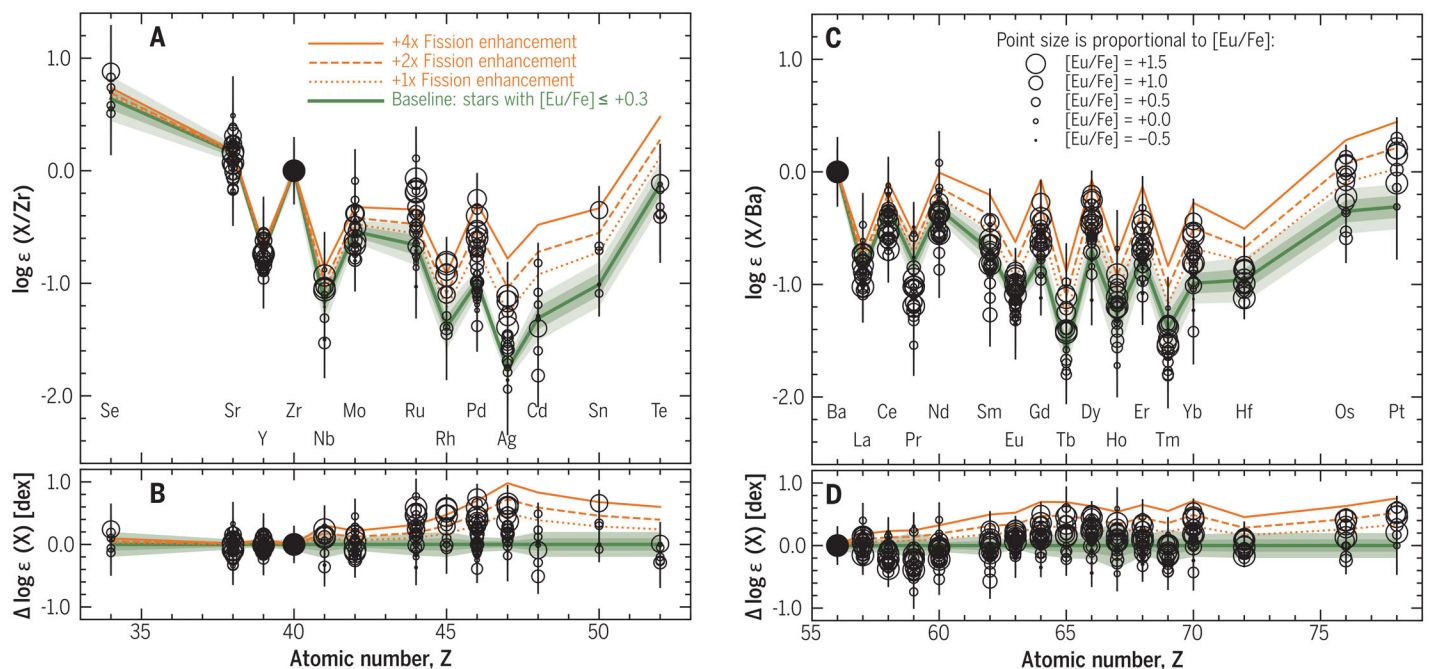
Fig. 1. Observed abundance patterns compared with fission model predictions.
