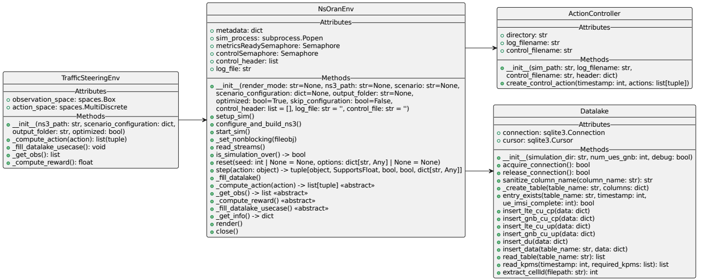
Fig. 1: Simplified Unified Modeling Language (UML) Diagram of the ns-O-RAN and the Traffic Steering environments
