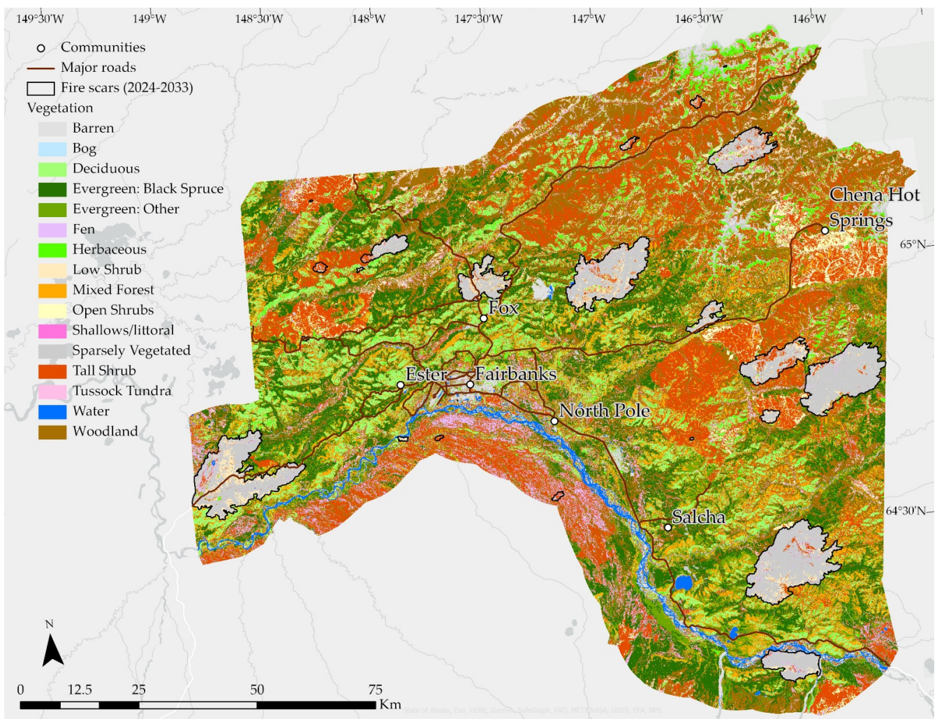
Figure 7. 2034 landcover for Fairbanks with 2024–2033 modeled fire perimeters.
