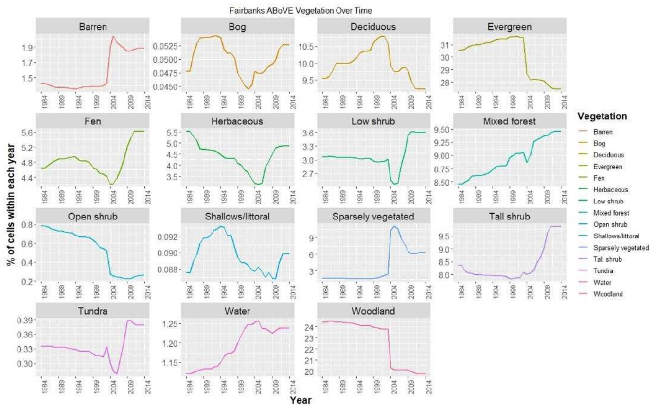
Figure A1. Changes in land cover in the Fairbanks study area as identified in ABoVE by year.
