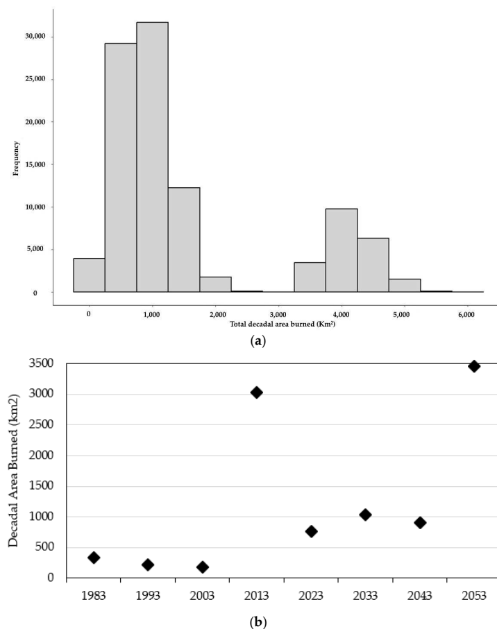
Figure 6. Area burned trends for the Fairbanks study area. (a) Results of 100,000 Monte Carlo simulations of decadal area burned (in km 2 ) based on random combination of historic annual area burned from the period 1950–2021. Here, frequency represents the number of simulations. (b) Historic (1974 to 2022) and simulated (2023–2053) decadal area burned (in km 2 ), years on the x -axis indicate when the decade ended, so 1983 includes area burned from 1974 to 1983.
