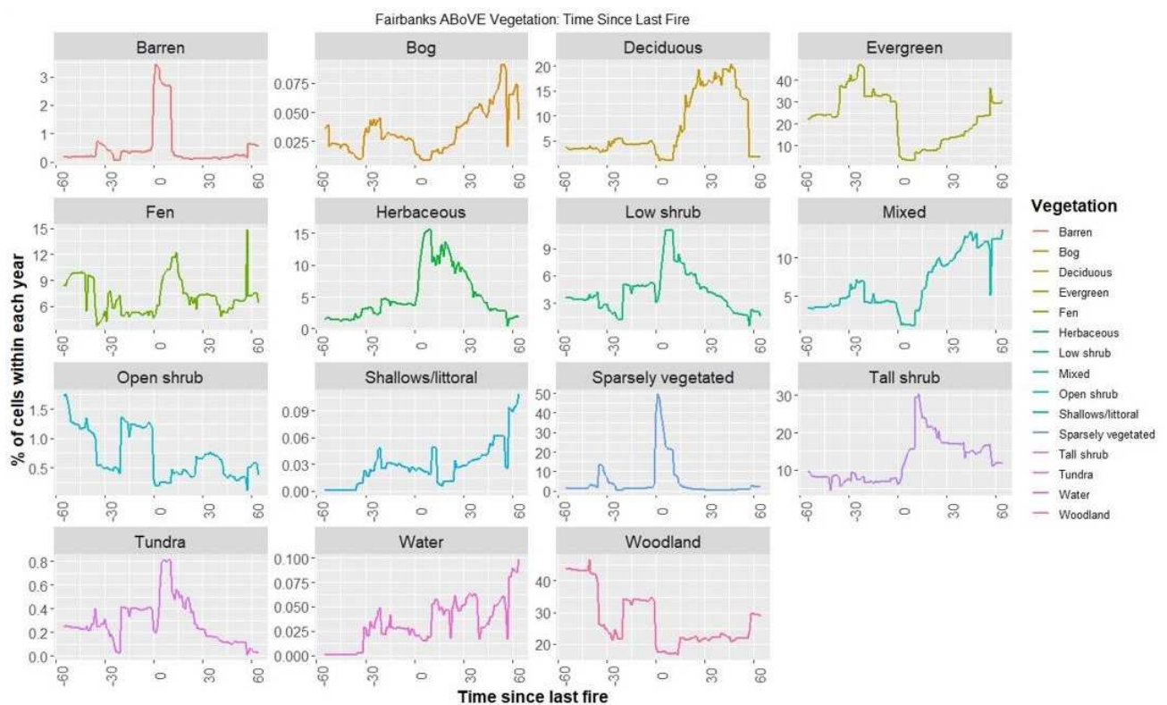
Figure A2. Changes in land cover in the Fairbanks study area as identified in ABoVE pixels of time since the last fire.
