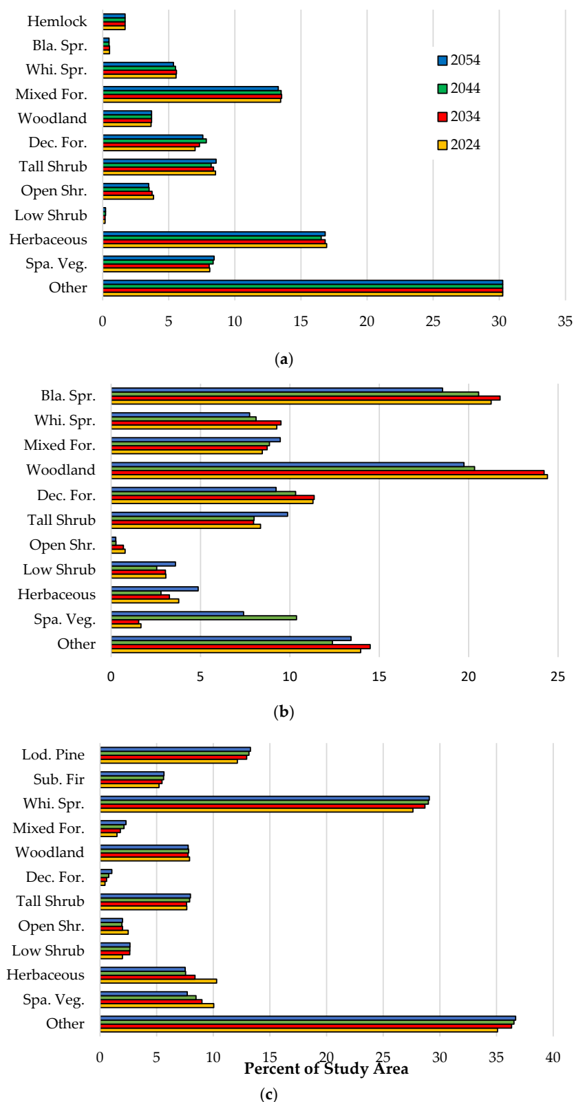
Figure 8. Predicted future landcover in the (a) Anchorage, (b) Fairbanks, and (c) Whitehorse study areas. Units are given as percent of study area. Here, Bla. Spr. = Black Spruce, Whi. Spr. = White Spruce, Mixed For. = Mixed Forest, Dec. For. = Deciduous Forest, Open Shr. = Open Shrubs, Spa. Veg. = sparsely vegetated, Lod. Pine = Lodgepole Pine, and Sub. Fir = Subalpine Fir. Other includes barren, bog, fen, NA, shallows/littoral, tussock tundra, and water.
