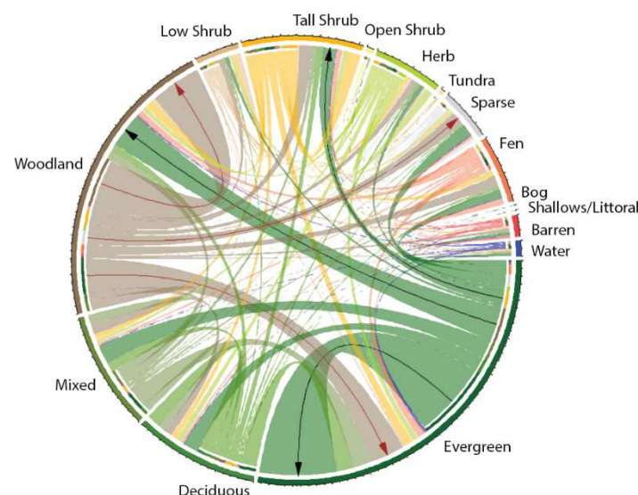
Figure 5. Landcover change from 1984 to 2014 in the Fairbanks study area. In this chord diagram, the size of each wedge indicates the proportion of the landscape and lines across the middle indicate transitions; 1984 landcover is set back from the edge, and arrows indicate change through time.
