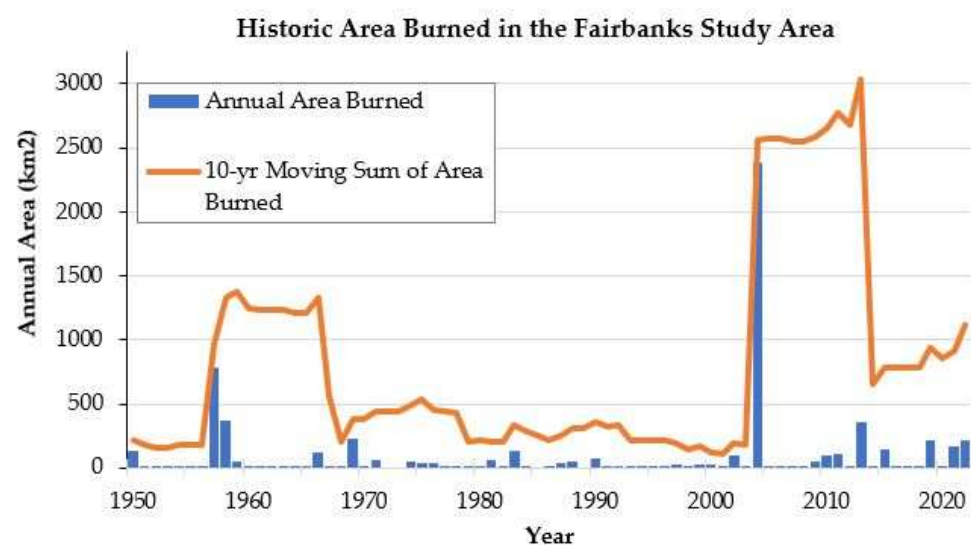
Figure 2. Historic area burned in the Fairbanks study area. Area burned (in km 2 ) is shown annually (blue bars) and as a 10-year moving sum (orange line).
