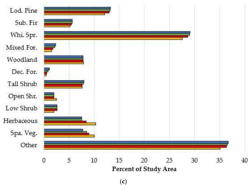
Figure 3. Landcover from 1984 to 2014 in the (a) Anchorage, (b) Fairbanks, and (c) Whitehorse study areas. Units are given as the percent of study area. Here Bla. Spr. = Black Spruce, Whi. Spr. = White Spruce, Mixed For. = Mixed Forest, Dec. For. = Deciduous Forest, Open Shr. = Open Shrubs, Spa. Veg. = sparsely vegetated, Lod. Pine = Lodgepole Pine, and Sub. Fir = Subalpine Fir. Other includes barren, bog, fen, NA, shallows/littoral, tussock tundra, and water.
