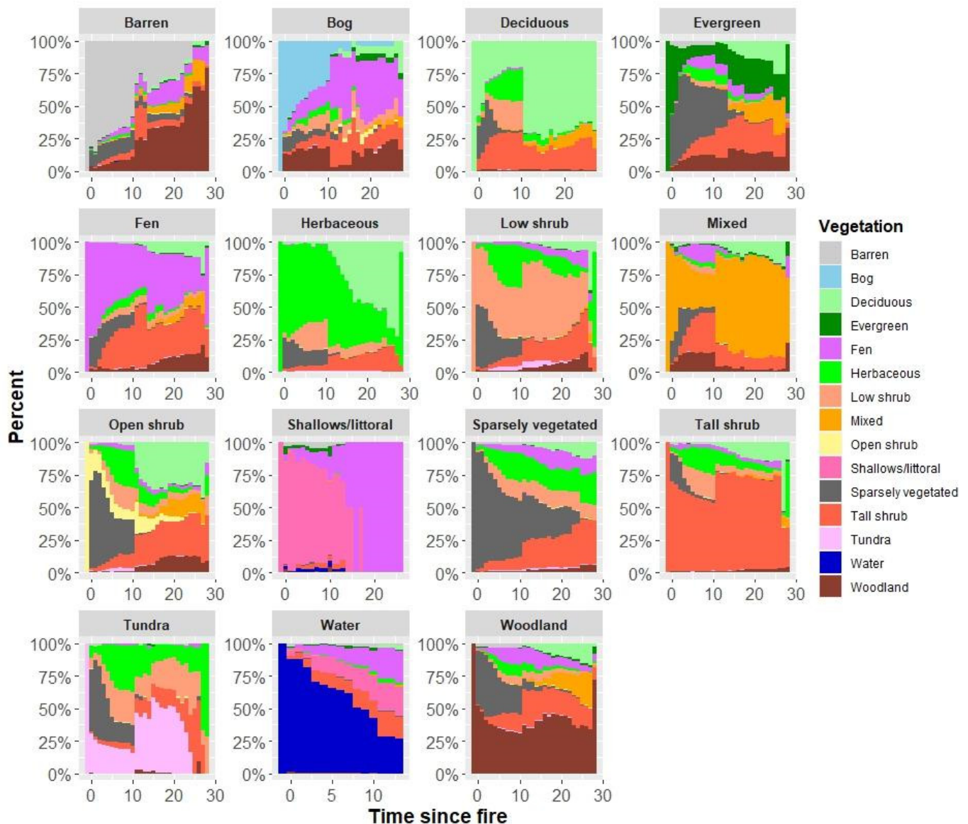
Figure 4. Vegetation changes after fire (year 0) in the Fairbanks study area based on ABoVE data and organized by pre-fire vegetation type. Only burns between 1985 and 2021 were used. Pre-fire vegetation for burns after 2014 was assumed to be the same as 2014 counts. Actual pixel counts decrease with time since fire and are provided in Figure A3.
