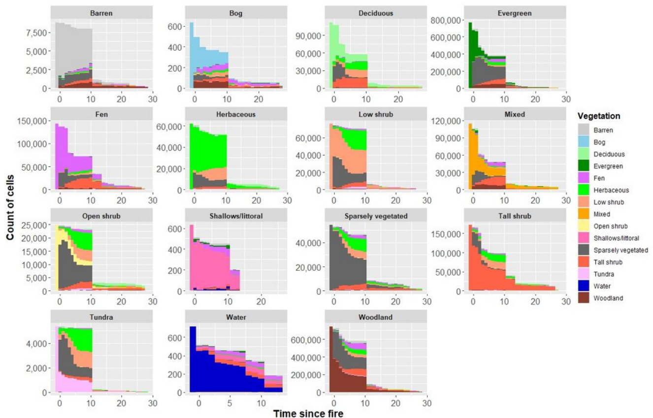
Figure A3. Cell counts of the vegetation present after a fire based on pre-fire vegetation type. Only burns between 1985 and 2021 were used. Pre-fire vegetation for burns after 2014 was assumed to be the same as 2014 counts.
