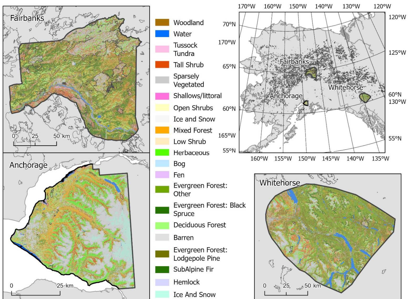
Figure 1. The three study areas in the western boreal zone. Vegetation is shown for 2014. Evergreen Forest: Black Spruce is only found in Fairbanks and Anchorage; Hemlock is only found in Anchorage; and SubAlpine Fir and Evergreen Forest: Lodgepole Pine are only found in Whitehorse. Thin gray outlines delineate fire perimeters for 1980 to 2019 in Alaska and from 1980 to 2022 in the Yukon.
