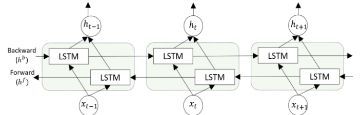
Figure 2: Architecture of the Bi-LSTM network.
