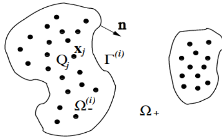
Figure 1: A schematic diagram of charged molecules immersed in an aqueous solvent. The region of solvation \Omega is divided by the solute-solvent interface (i.e., dielectric boundary) \Gamma into the solute region \Omega_- and the solvent region \Omega_+ . The solute region \Omega_- , which can have multiple connected subregions, contains all the solute atoms x_i carrying partial charges Q_i ( i = 1, \dots, N ). The unit normal n at \Gamma points from \Omega_- to \Omega_+ .
