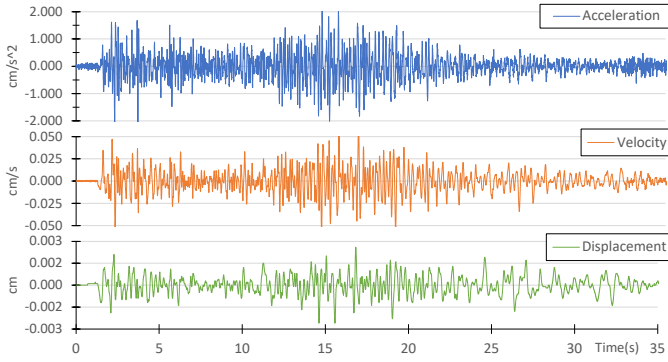
Fig. 2. Accelerographic data (one component)
