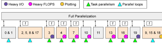
Fig. 10. Full parallelization: all stages are executed in parallel.
