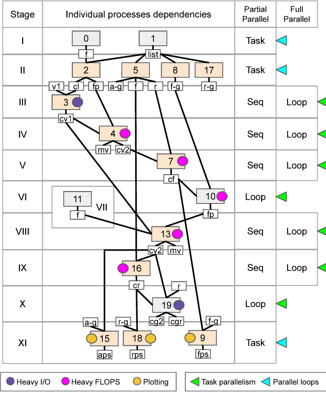
Fig. 9. Processes reordering into 11 stages. Parallel approaches for each individual stage (rows) for the first and second parallel versions (right-most columns) are detailed, as well as input/output dependencies for each process.
