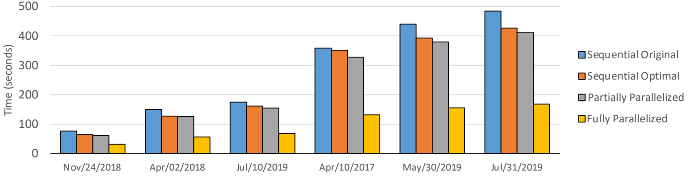
Fig. 12. Speedup per Event: execution time is proportional to the number of data points in each seismic event.
