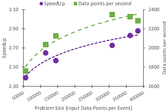
Fig. 13. Overall speedup in parallel accelerographic records processing: problem size vs. speedup (purple) and vs. data points per second (green).
