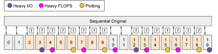
Fig. 6. Original sequential version: processes overview
