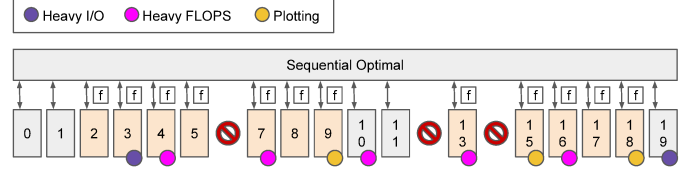
Fig. 7. Optimized sequential version: processes overview
