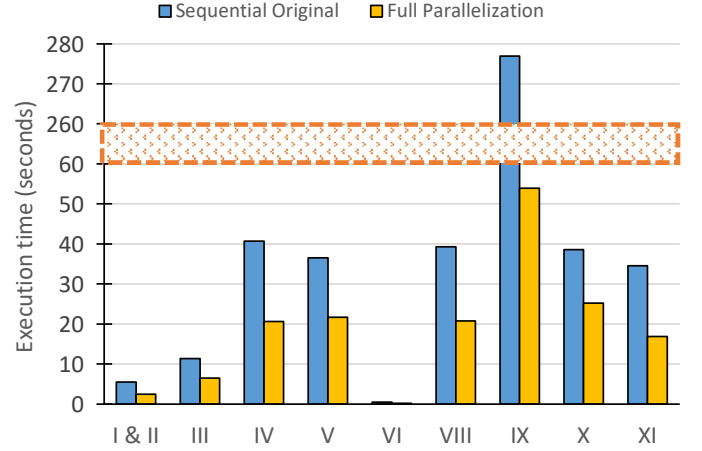
Fig. 11. Speedup per individual Stage (19 Files, 384k Data points)
