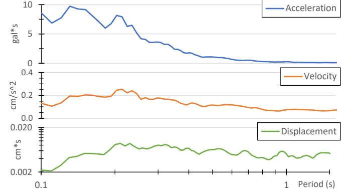
Fig. 4. Response spectrum (one component)
