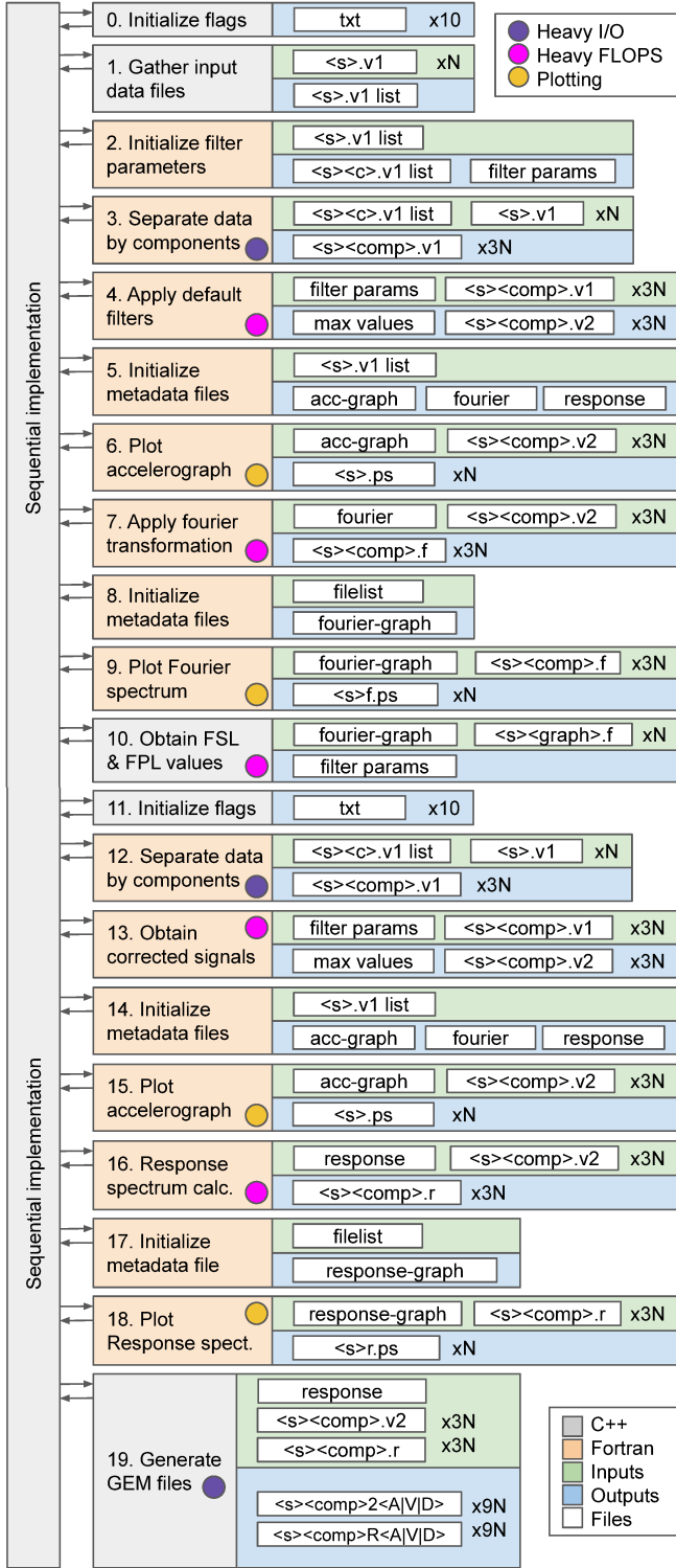
Fig. 5. Sequential accelerographic records processing implementation
