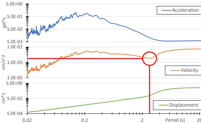
Fig. 3. Inflection point in the velocity Fourier spectrum (one component), indicates the values of the FPL & FSL signal filtering parameters.
