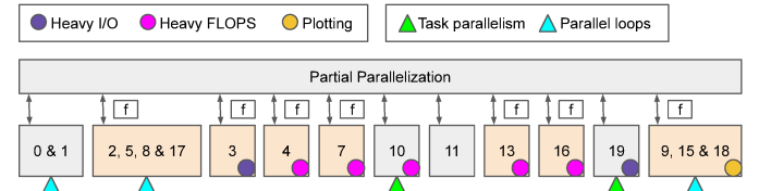
Fig. 8. Partial parallelization: 5 out of 11 stages are executed in parallel.
