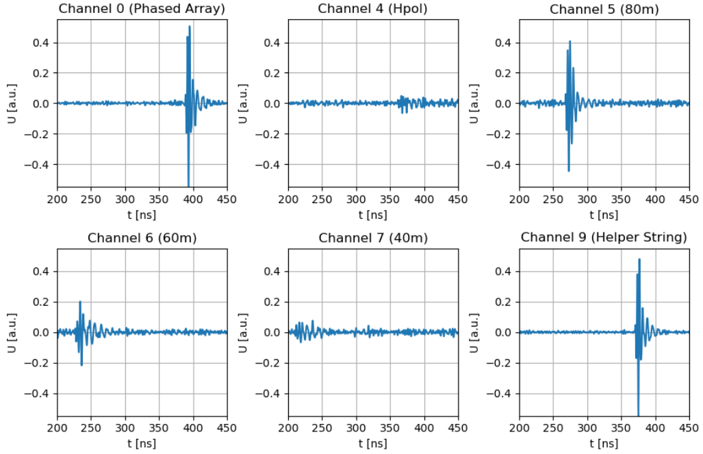
Figure 2: Signals from the pulser on one of the helper strings recorded by an RNO-G station. Channel 0 is one of the four antennas that make up the phased array. Channel 4 is one of the horizontally polarized antennas on the power string . Channels 5, 6, and seven are vertically polarized antennas on the power string at 80 m, 60 m and 40 m, respectively. Channel 9 is one of the vertically polarized antennas on a helper string .
