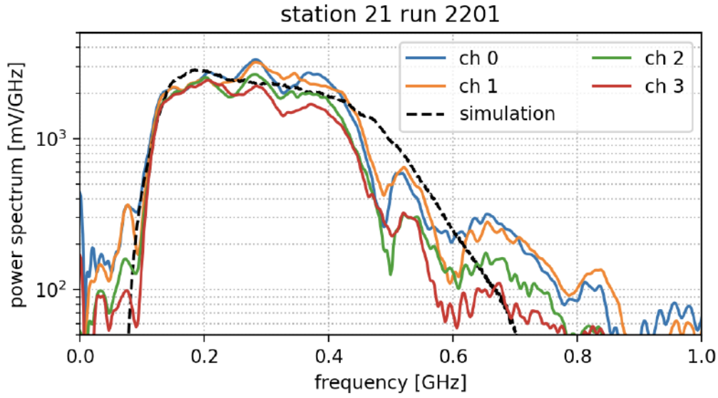
Figure 3: Spectrum of the signal from an in-situ pulser recorded by the phased array channels of RNO-G station 21, along with the simulated spectrum, rescaled to match the measurements.
