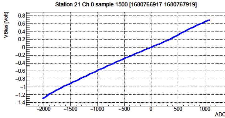
Figure 4: Example of a digitizer calibration, showing the relation between the ADC count and the bias voltage that is applied to the ADC.
