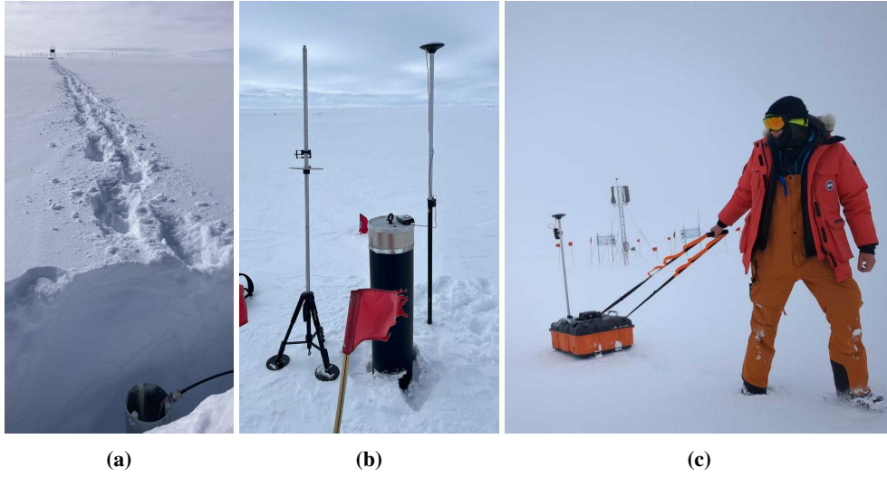
Figure 1: RNO-G calibration measurements in the field: Temporary surface pulser at an RNO-G station (a). GPS survey (b). Survey using ground penetrating radar (c)
