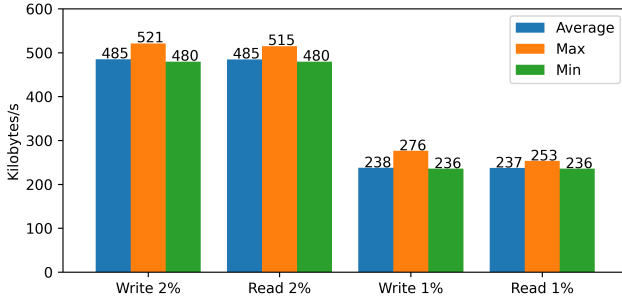
Fig. 16: Average, Maximum and Minimum USB Round Trip Throughputs with I/O VCPU Utilizations of 1% and 2%
