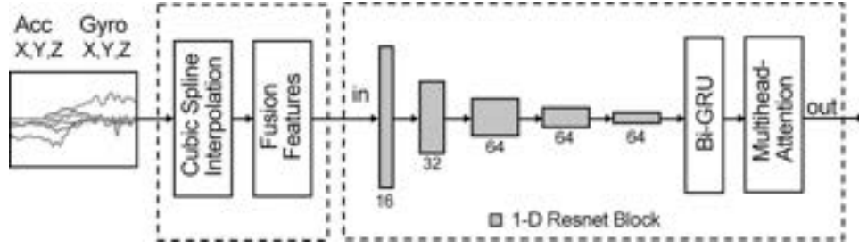
Fig. 8. Feature Extraction.
