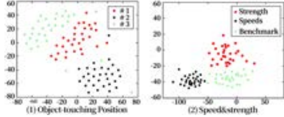
Fig. 5. T-SNE Visualization for (1) different object-touching positions and (2) different grab speeds and forces, highlighting the potential impact of these factors on the performance of object recognition.
