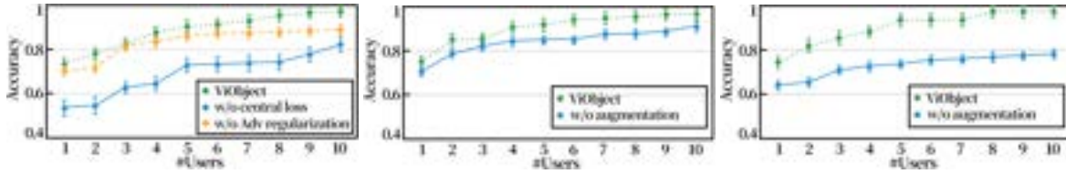
Fig. 17. Ablation study for different Fig. 18. Ablation study for different Fig. 19. Ablation study for different object-touching positions. grab-object speeds. grab-object strengths.
