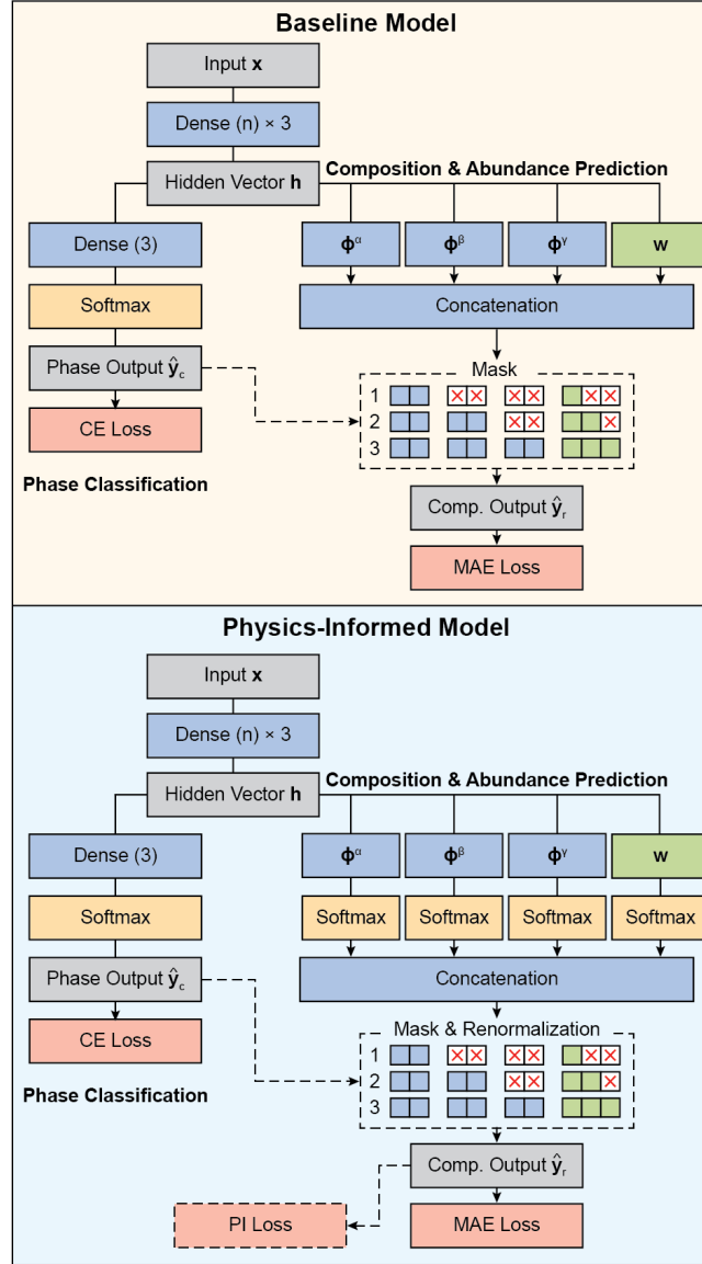
Figure 2: Architectures of the machine learning models. In both the baseline and physics-informed (PI) models, the parameter vector x is fed into the model to produce an intermediate hidden vector h . The hidden vector h produces two outputs: (1) a phase classification probability vector \hat{y}_c , trained with cross-entropy (CE) loss, and (2) an equilibrium composition and abundance vector \hat{y}_r , trained with mean absolute error (MAE) loss. Softmax activation is applied in PI models to ensure that the equilibrium composition and abundance vectors sum to unity. Optional functionalities (indicated by dashed lines and boxes) include a “mask”, activated based on \hat{y}_c , which sets corresponding elements in \hat{y}_r to zero if an input is classified as one- or two-phase. For PI models, softmax renormalization is applied to the masked abundance to ensure the sum equals unity. Additionally, in PI models, a PI composite loss can be incorporated alongside the MAE loss during training for \hat{y}_r prediction.
