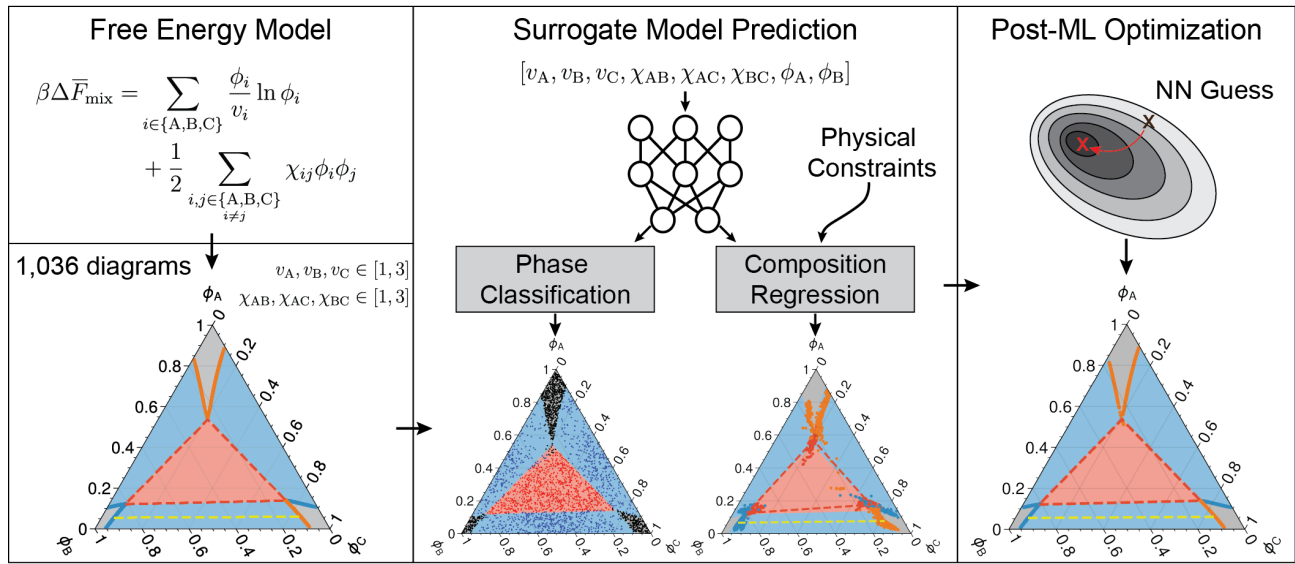
Figure 1: Strategy for multi-component phase-coexistence prediction using machine learning. 1,036 ternary phase diagrams are generated using the algorithm arc continuation algorithm (Equations 6-8) and convex hull construction algorithm, 39 and are used as training data for a physics-informed machine learning (ML) model to classify phase regions and predict equilibrium phase compositions. The ML predictions serve as initial guesses for the Newton-CG method to obtain equilibrium composition predictions.
