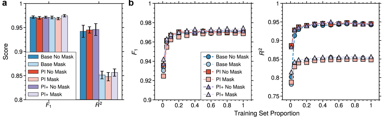
Figure 4: Impact of physical constraints and data size on phase-coexistence prediction. a) Comparison of test set phase classification F_1 and equilibrium composition prediction R^2 across baseline (base), physics-informed (PI), and augmented PI (PI+) models, with and without classification masks, using five-fold cross-validation (CV). Bars represent mean values, and error bars indicate standard deviations. b) The impact of training data size on model performance. Each dot represents the average score calculated across the five-fold CV.
