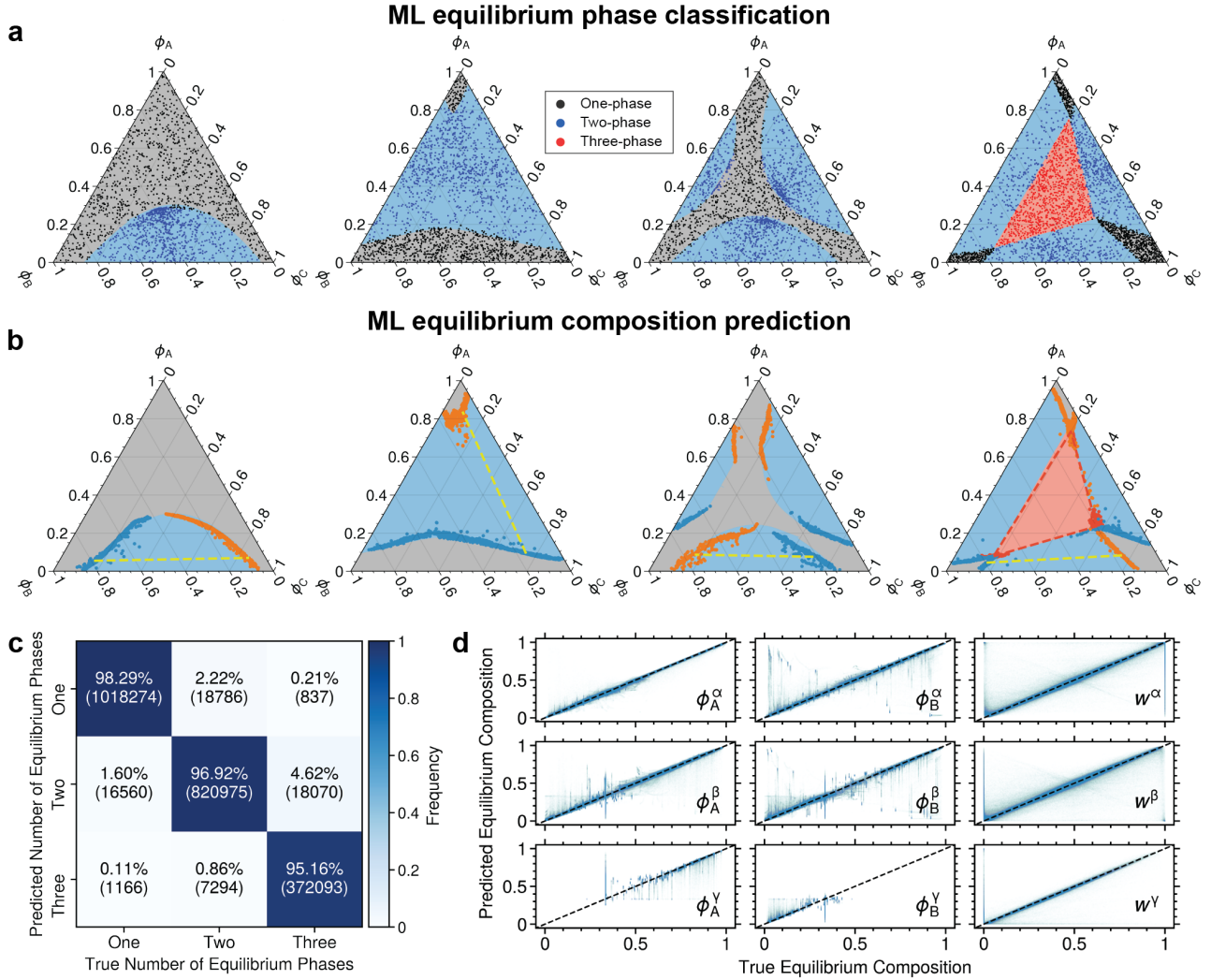
Figure 3: A summary of the baseline model. a) Classification of the number of coexisting phases. The background color in all phase diagrams denotes the ground truth phase: gray (one-phase), blue (two-phase), and red (three-phase). Scatter points represent the predicted phase splits for a given initial composition, and the legend colors indicate the types of predicted splits. b) Predicted equilibrium compositions. Blue and orange scatter points represent two-phase equilibrium compositions. The yellow dashed line is a tie line for the two-phase split. Red scatter points depict composition that split into three phases. The red dashed triangle connects the three compositions at equilibrium. c) Confusion matrix for the predicted number of equilibrium phases. Diagonal entries represent correctly classified instances, while off-diagonal entries represent misclassifications. d) Parity plot for predicted equilibrium compositions. The diagonal dashed line represents perfect performance.
