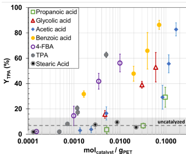
Figure 3. Influence of carboxylic acid catalyst loading on the TPA yield from PET hydrolysis (200 °C, 2 h, 1/10 mass ratio PET/water). The dashed line represents the TPA yield average without catalyst, and the shaded area the standard deviation.
