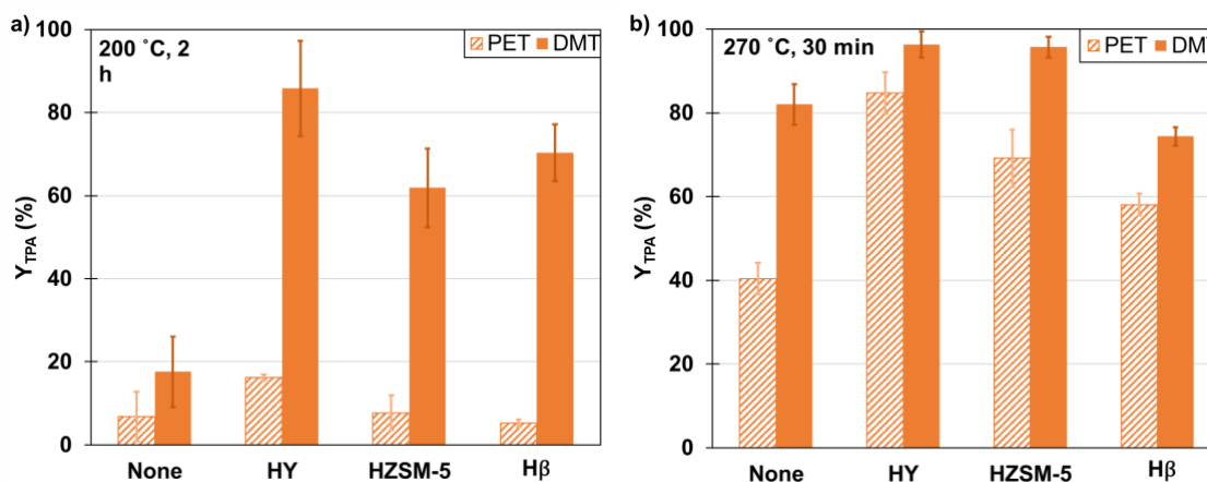
Figure 1. TPA yield from hydrolysis of PET chips and DMT (1/5/50 mass ratio of zeolite/PET or DMT/water). a.) 200 °C, 2 h, b.) 270 °C, 30 min.
