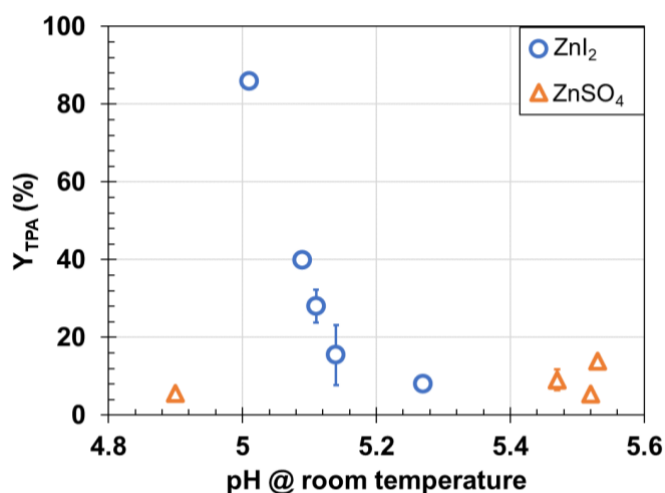
Figure 4. Effect of ZnI 2 and ZnSO 4 on TPA yield from PET hydrolysis (200 °C, 2 h, 1/10 mass ratio PET/water).
