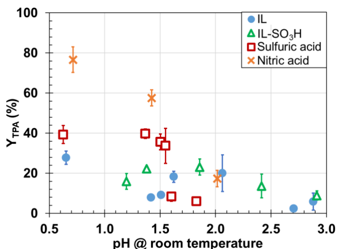
Figure 2. Influence of pH (measured at room temperature) on the TPA yield from PET hydrolysis with sulfuric acid, nitric acid, and ionic liquids (200 °C, 2 h, and 1/10 mass ratio PET/water).
