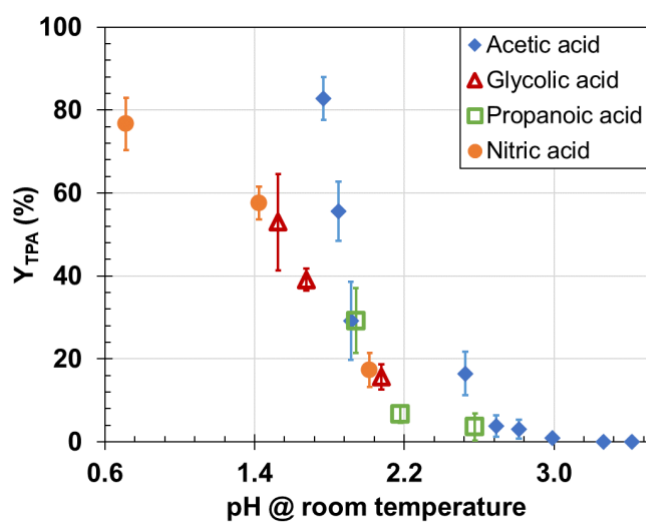
Figure 5. Effect of pH on TPA yield from PET hydrolysis with different aliphatic carboxylic acids and nitric acid (200 °C, 2 h, 1/10 mass ratio PET/water).
