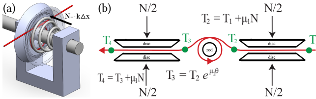
Figure 4: SPEERLoom’s tensioning mechanism consisting of (a) two tensioning disks, a conical spring, and a spacer with the yarn (red) wrapped around the rod. (b) Model of the tension of the system.
