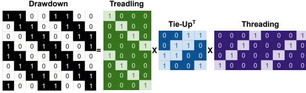
Figure 13: An image showing the matrix multiplication of weaving draft elements for an example 2x2 twill pattern.
