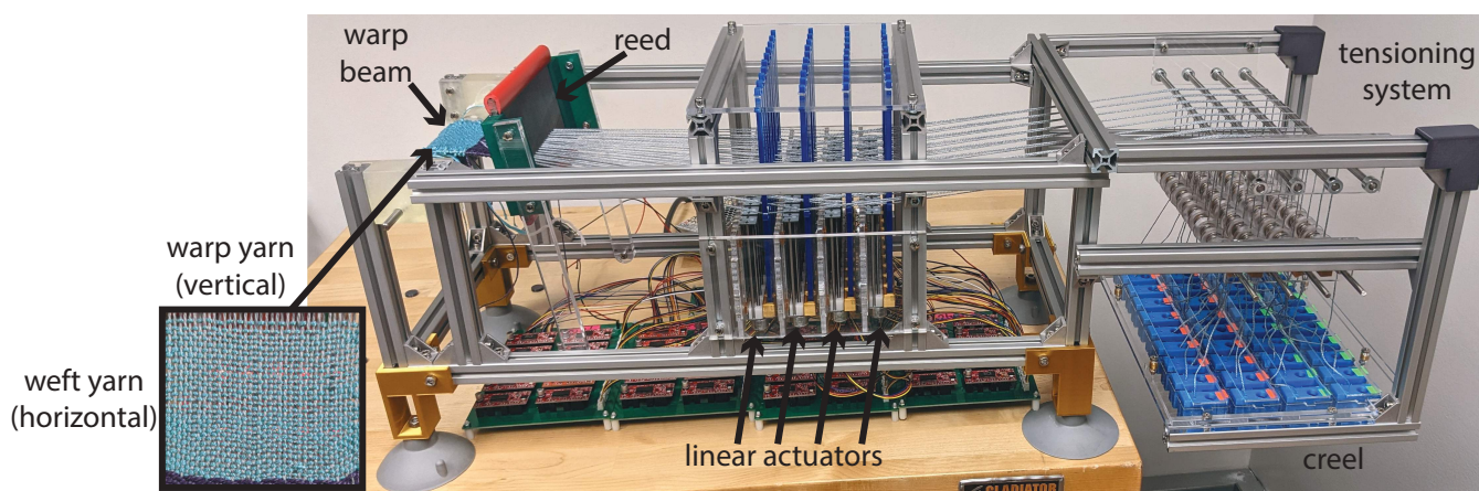
Figure 1: Semi-automated Pattern Executing Educational Robotic Loom (SPEERLoom): An open-source robotic Jacquard loom kit for use in interdisciplinary collegiate classrooms
