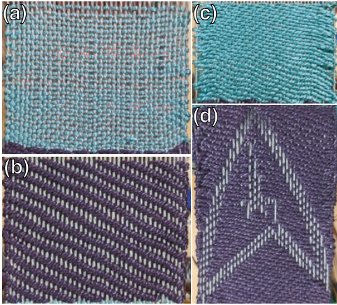
Figure 7: Cloth woven on SPEERLoom: (a) Plain Weave, (b) Twill Weave, (c) Satin Weave, (d) Custom Jacquard Weave.
