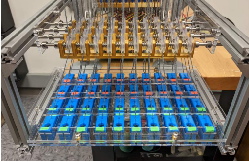
Figure 3: SPEERLoom’s novel tensioning system and creel. The creel has 40 individual cases with bobbins holding \approx 6 meters of yarn. The yarns are then passed through the tensioning system. Each frame has its own tensioning rod.
