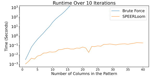
Figure 15: The graph shows the run time of each algorithm over 10 iterations of the algorithm as the number of columns in the pattern is increased.
