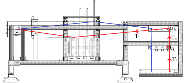
Figure 5: Different warp yarn positions in SPEERLoom. Each heddle can be either raised or lowered, with the same amount of tension pulled on the warp yarn in either position. Yarns (blue and red) pass through the tensioning system and over the guiding rods before going through the heddles.
