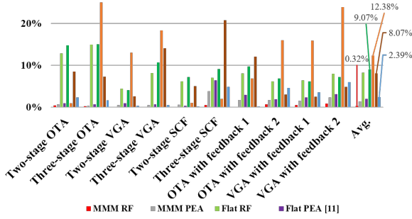
Fig. 7: UGF (Unity Gain Frequency) estimation errors.
