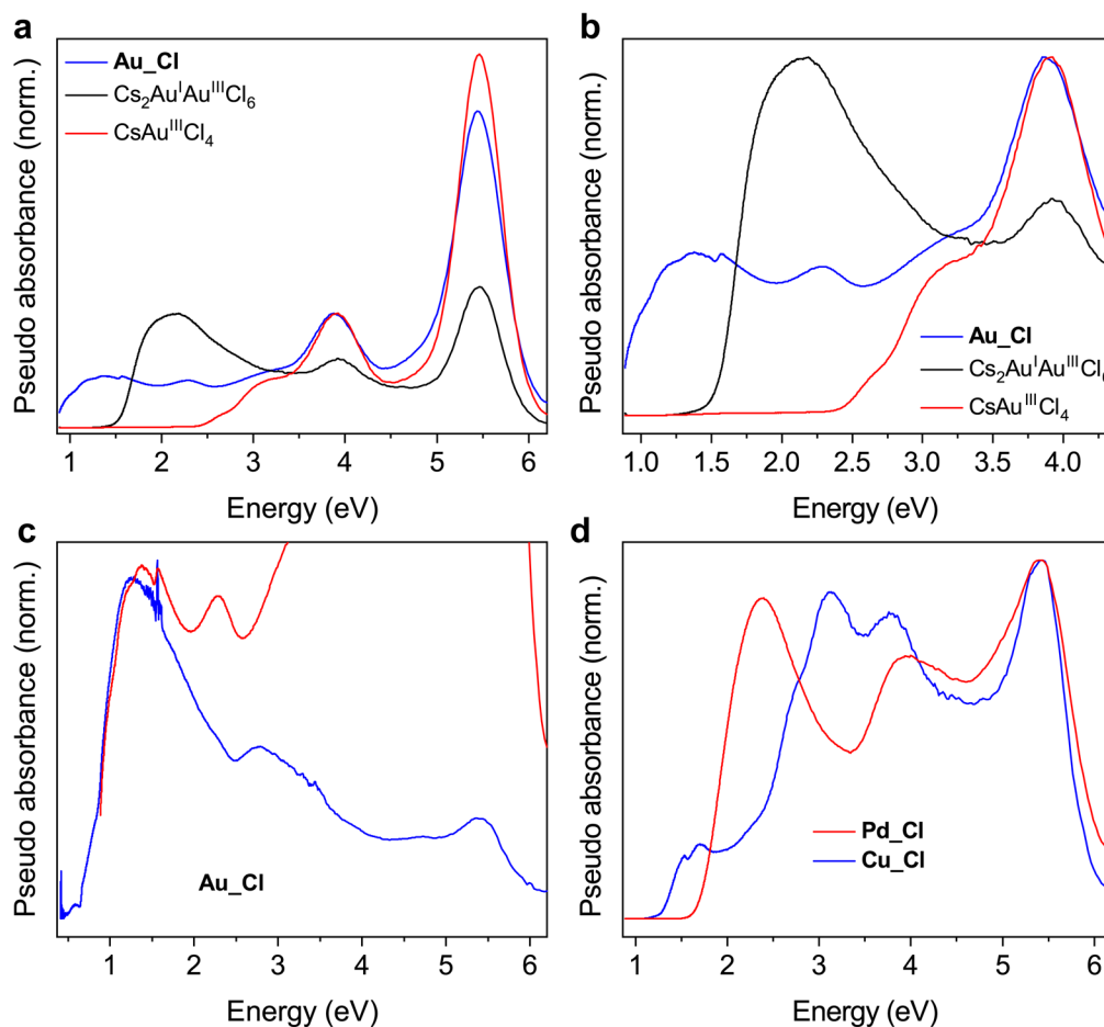
Extended Data Fig. 9 | UV-vis-NIR absorbance spectra of crystals pulverized into a mull with BaSO 4 and converted from diffuse reflectance spectra using the Kubelka–Munk transformation. a, b Spectra normalized to the highest point at or below 4.5 eV. c , Spectra normalized to align near the first absorption peak. The same spectra are shown in (a) and (b) with two different energy
