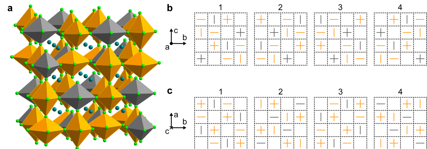
Extended Data Fig. 1 | Representation of the X-ray diffraction single-crystal structure of Pd-Cl. a , A 3D representation where turquoise and light green spheres represent Cs and Cl atoms, respectively, and gold and grey octahedra represent \text{Au}^{\text{III}}\text{Cl}_6 and \text{Pd}^{\text{II}}\text{Cl}_6 , respectively, and the viewing direction is shown by the coordinate system in panel (b). b,c , 2D representations of the crystal structure of Pd-Cl where the short, equatorial bonds of the axially elongated \text{Au}^{\text{III}}\text{Cl}_6 and \text{Pd}^{\text{II}}\text{Cl}_6 octahedra are represented by gold and grey lines, respectively.
