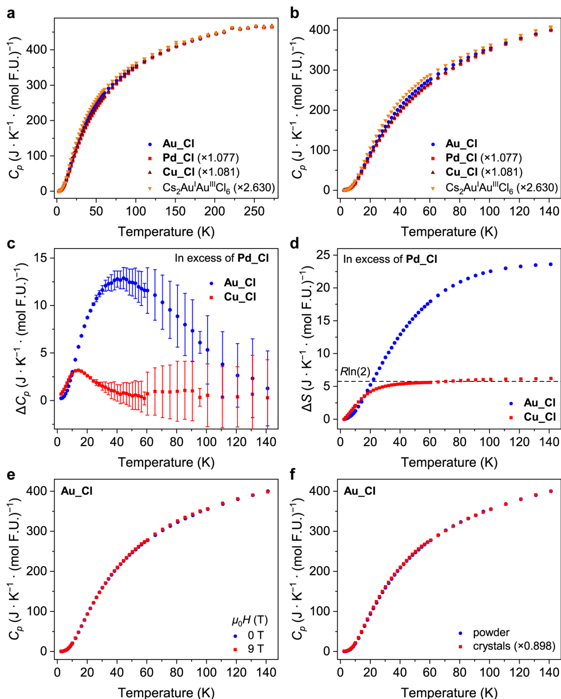
Extended Data Fig. 7 | Heat capacity measurements. a , Heat capacity normalized at high temperatures (~200–275 K). b , A magnified region of the same data presented in (a). The scaling factors denoted in the legends in (a,b) are probably due to inaccuracies in the measured sample masses and are scaled with respect to Au_Cl. c , The heat capacity in excess of that of Pd_Cl. The vertical bars represent the measurement uncertainty (1σ). d , Entropy ( \Delta S ) as extracted from the heat capacity in excess of that of Pd_Cl. The dashed horizontal line at R \ln(2) represents the expected excess entropy for a magnetic centre with spin S = 1/2 .
