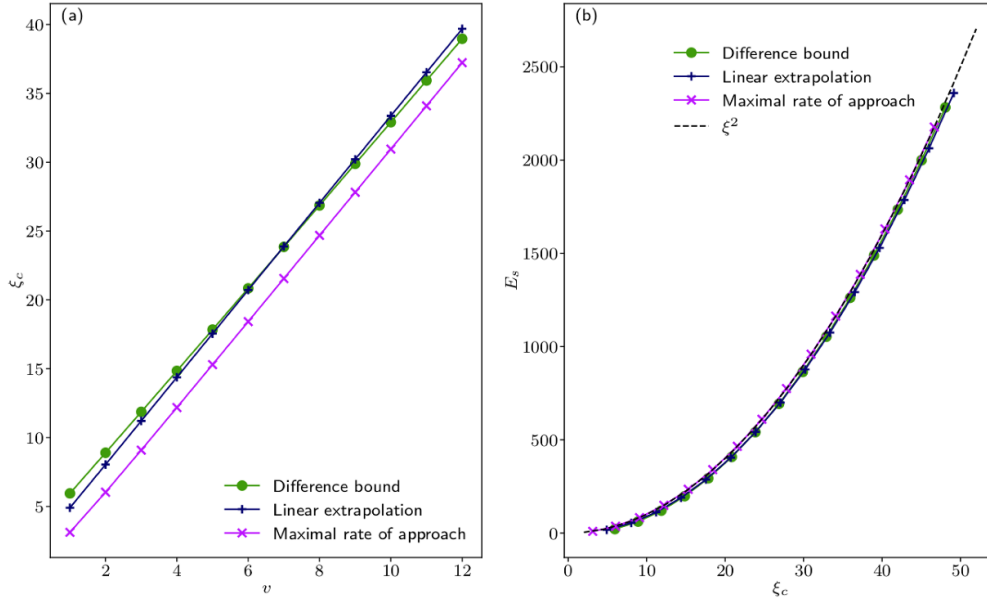
Figure 6. Panel (a): The values of the critical point \xi_c as a function of \nu as obtained by the three methods: maximal rate of approach (cross) [1], linear extrapolation (plus), and difference bound (circle). Panel (b): The values of the separatrix E_s as a function of \xi as obtained by the three methods of panel (a). The semiclassical result [37] is shown with a dashed line.
