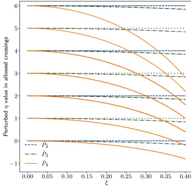
Figure 14. Behavior of the location of the degeneracies \pm m as a function of the strength \xi for the representations j = 1/2, 3/2, 5/2 , and 7/2 ( \eta = 0, 2, 4, 6 ) for \hat{P}_2 , \hat{P}_3 , and \hat{P}_4 and the representations j = 1, 2 , and 3 ( \eta = 1, 3, 5 ) for \hat{P}_3 and \hat{P}_4 .
