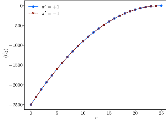
Figure 2. Eigenvalues of the operator -\hat{C}_2 as a function of v for N = 50 . Each point is doubly degenerate, \pi' = \pm , except v = N/2 = 25 .
