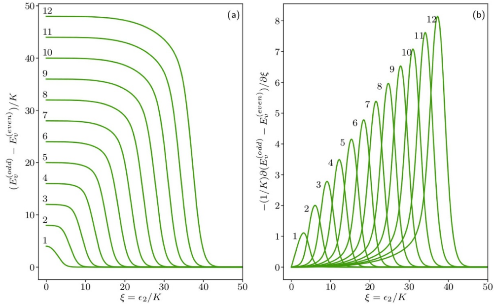
Figure 5. Panel (a): The gap (E_v^{(odd)} - E_v^{(even)})/K as a function of \xi for v = 1, \dots, 12 . Panel (b): The derivative of the gap -(1/K) \partial(E_v^{(odd)} - E_v^{(even)})/\partial \xi as a function of \xi for v = 1, \dots, 12 . The critical value \xi_c is the value of \xi at the maximum of the derivative [9]. The gaps go to zero as the separatrix is crossed for each v as a function of \xi . To the right of the separatrix, states are doubly degenerate with E_v^{(odd)} = E_v^{(even)} (parity \pm ).
