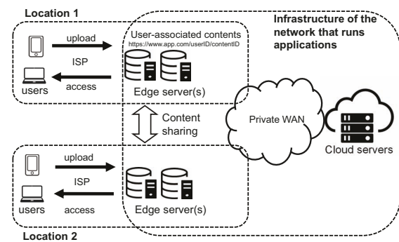
Figure 1: Infrastructure of edge content caching.
