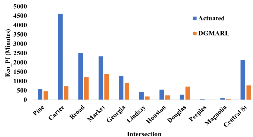
Figure 7. 55.38% improvement of overall Eco_PI in one 24-hour test duration.
