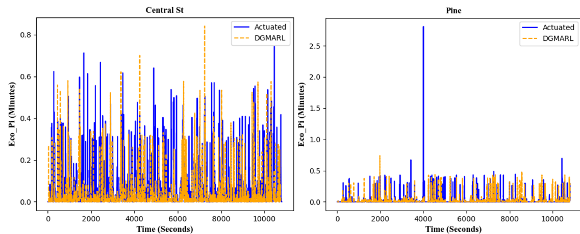
Figure 11. Variation of Eco PI during simulation period for Actuated and DGMARL.
