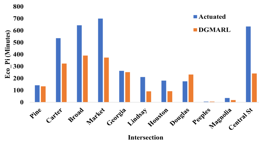
Figure 8. 38.94% improvement in average of Eco_PI during PM-peak hour with 10 runs of tests.
