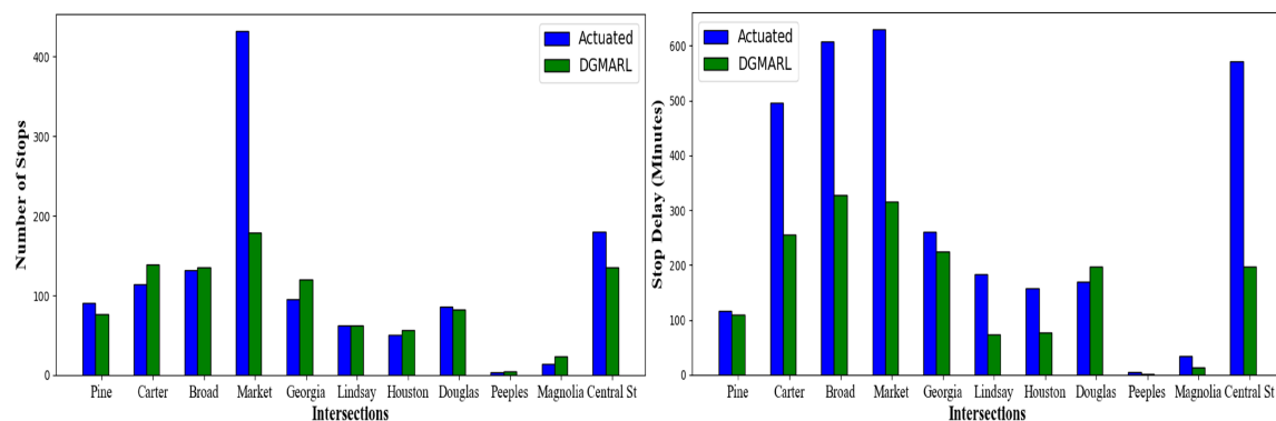
Figure 10. 13% reduction in stops and 43.29% reduction in stop delays during PM-peak hour in one run of the test.
