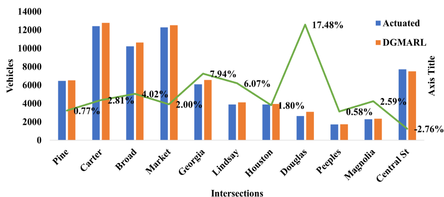
Figure 13. PM-peak hour traffic throughput in the MLK Smart Corridor: Actuated vs DGMARL.
