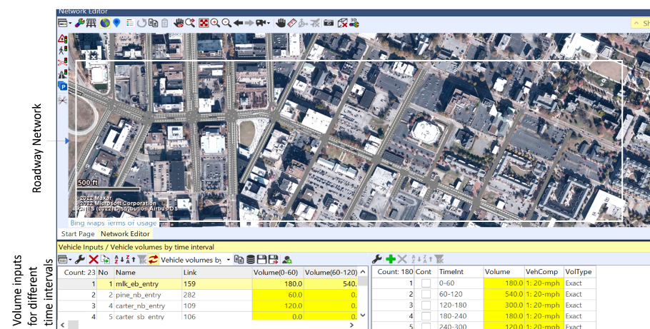
Figure 6. MLK Smart Corridor in PTV-Vissim showing roadway network layout and vehicle volume inputs per time interval.
