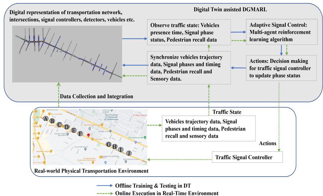
Figure 3. Digital Twin assisted DGMARL Learning.
