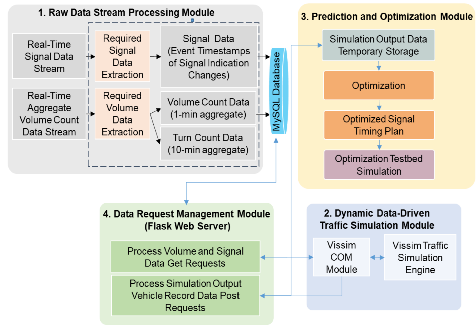
Figure 1. Digital Twin Architecture.
