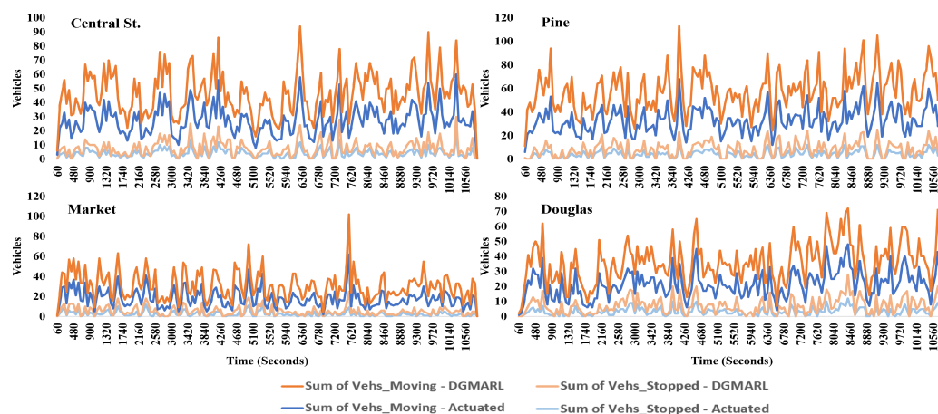
Figure 14. Stopped vs Moving Vehicles in PM-peak hour traffic.
