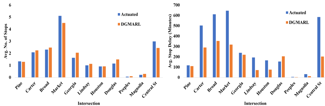
Figure 9. 42.78% reduced in the average of stop delays and 0.82% increase in the average number of stops during Pm-peak hour with 10 runs of tests.
