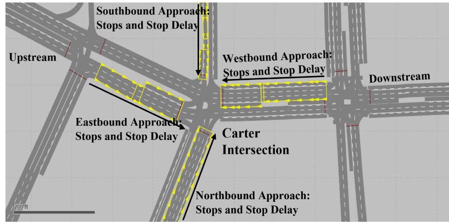
Figure 5. Vehicles Stops and Stop Delays at each approach.
