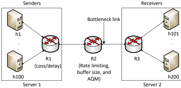
Figure 3: Topology used for the evaluations.
