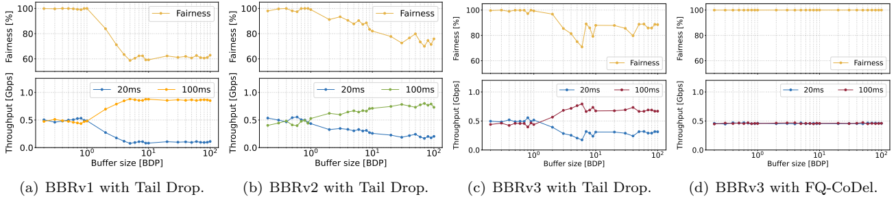
Figure 5: Fairness index and throughput as a function of the buffer size for a pair of competing flows: one with a 20ms propagation delay and the other with a 100ms propagation delay.
