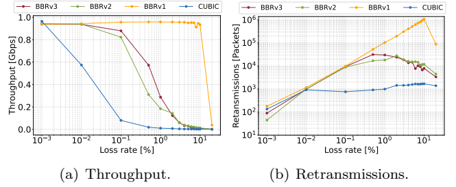
Figure 7: Throughput and retransmissions as a function of the packet loss rate.
