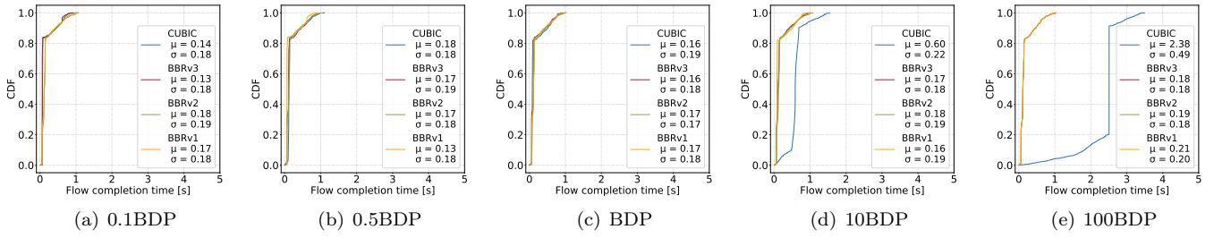
Figure 12: The Cumulative Distribution Function (CDF) for the Flow Completion Time (FCT) of short flows using CUBIC, BBRv1, BBRv2, and BBRv3 is analyzed while these flows compete with a long flow. It is important to note that the CDF curves for BBRv1, BBRv2, and BBRv3 overlap.
