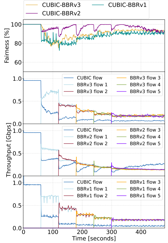
Figure 9: Throughput and fairness index over time as a CUBIC flow interacts with successive BBRv3, BBRv2, and BBRv1 flows.
