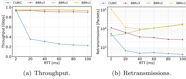
Figure 8: Throughput and retransmission of CUBIC, BBRv1, BBRv2, and BBRv3 as a function of the RTT.
