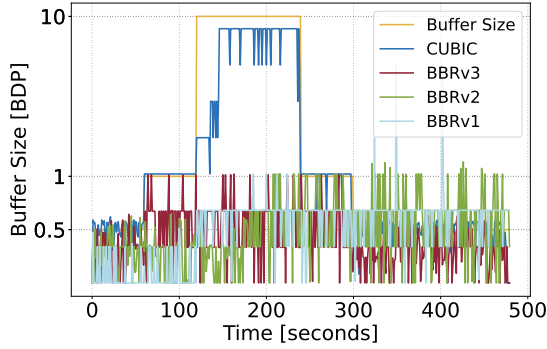
Figure 6: Queue occupancy for different buffer sizes for CUBIC, BBRv1, BBRv2, and BBRv3.
