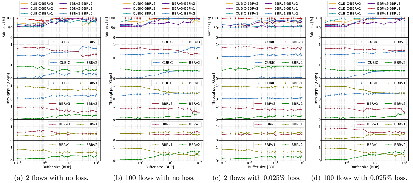
Figure 4: Fairness index and throughput with respect to the buffer size in four different scenarios: (a) Two competing flows without packet losses. (b) One hundred flows equally divided in a 50:50 ratio without packet losses. (c) Two flows with 0.025% packet losses. (d) One hundred flows equally divided in a 50:50 ratio with 0.025% packet losses.
