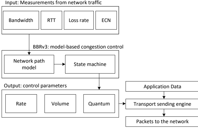
Figure 1: High-level architecture of BBRv3.
