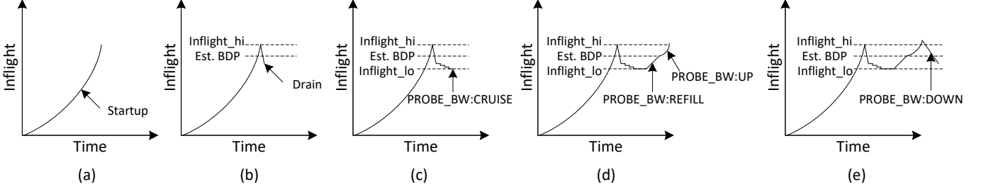
Figure 2: Life cycle of a BBRv3 flow and its five phases: (a) STARTUP , (b) DRAIN , (c) PROBE_BW:CRUISE , (d) PROBE_BW:REFILL and PROBE_BW:UP , and (e) PROBE_BW:DOWN .
