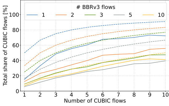
Figure 10: Bandwidth share for competing CUBIC and BBRv3 flows. The dashed lines show the ideal fair share and the solid lines show the measured share.
