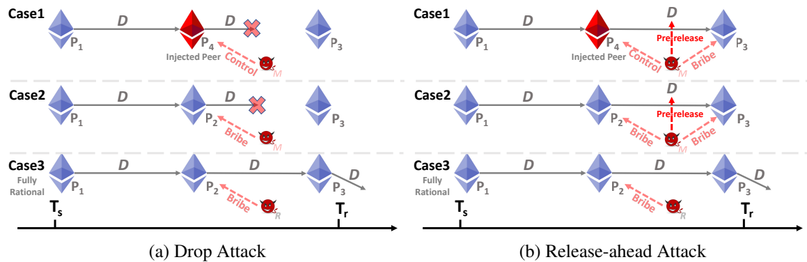
Fig. 2. Post-facto Attack Examples
