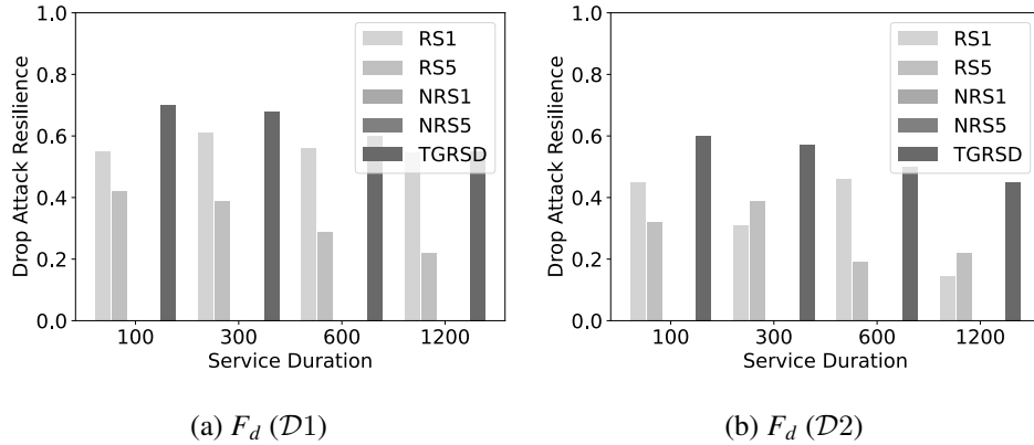
Fig. 10. F_d Evaluations under Timed-release Service Durations
