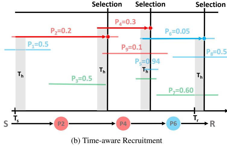
Fig. 4. Peer Recruitment Example
