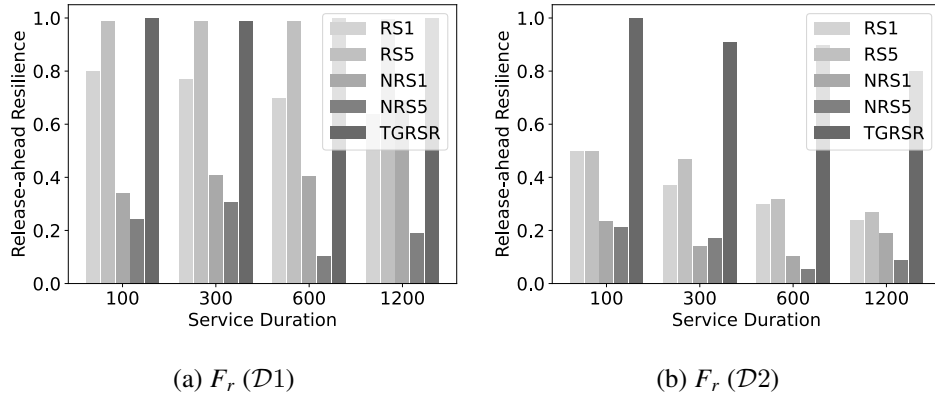
Fig. 9. F_r Evaluations under Different Timed-release Service Durations
