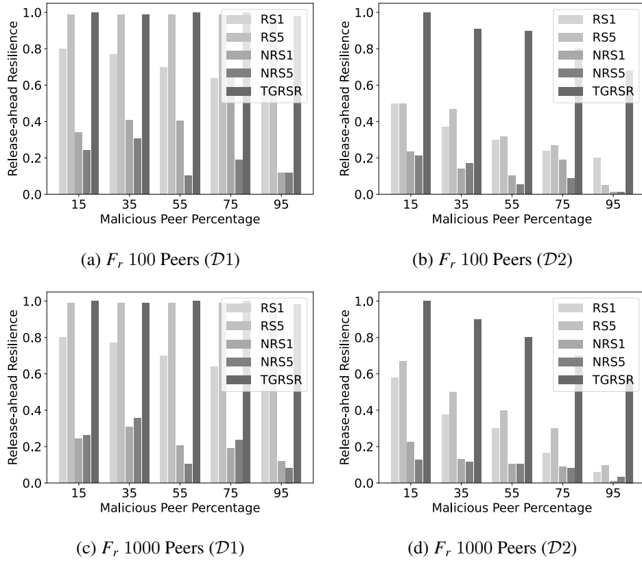
Fig. 7. F_r Evaluations under Different Malicious Peer Percentage
