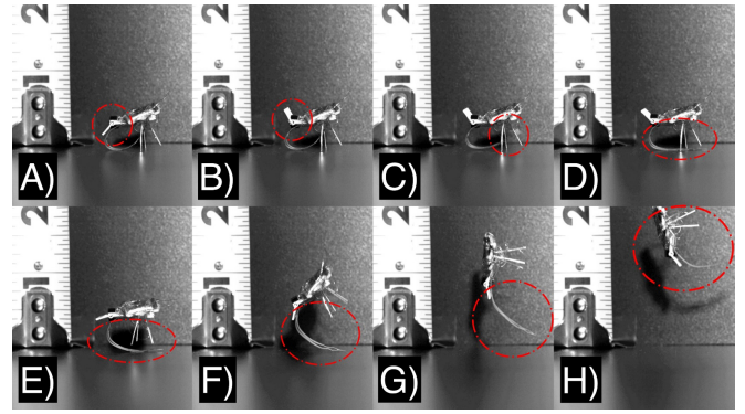
Fig. 6. A sequence of the microrobot unlatching and jumping. The microrobot was filmed at 10 000 fps, and keyframes with red markers showing A) no movement B) the actuator moving, C) spring unlatching, D) spring pushing against the ground, E) spring expansion, F) spring fully expanded, G) take-off from the ground, and H) ballistic motion. The entire sequence shown in these images occurs over 16.4 ms.
