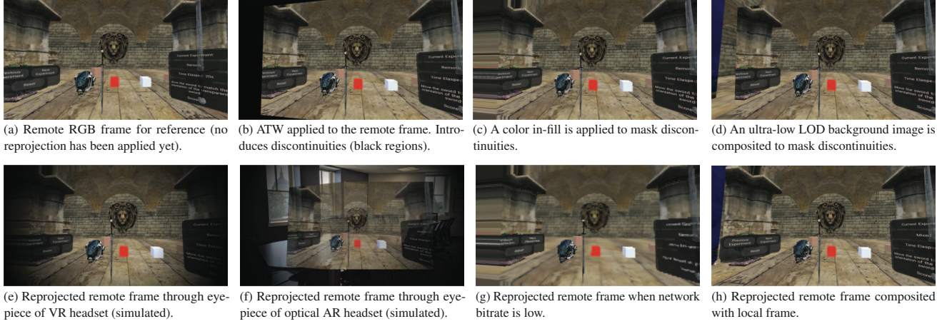
Figure 4: Results of applying ATW when remote and local cameras are not at the same pose. In all figures, all objects are rendered remotely, except for (h), which shows an outcome of RenderFusion. In (h), the background is local to reduce artifacts; helmet and blue cube are remote.
