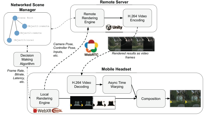
Figure 2: RenderFusion system architecture.
