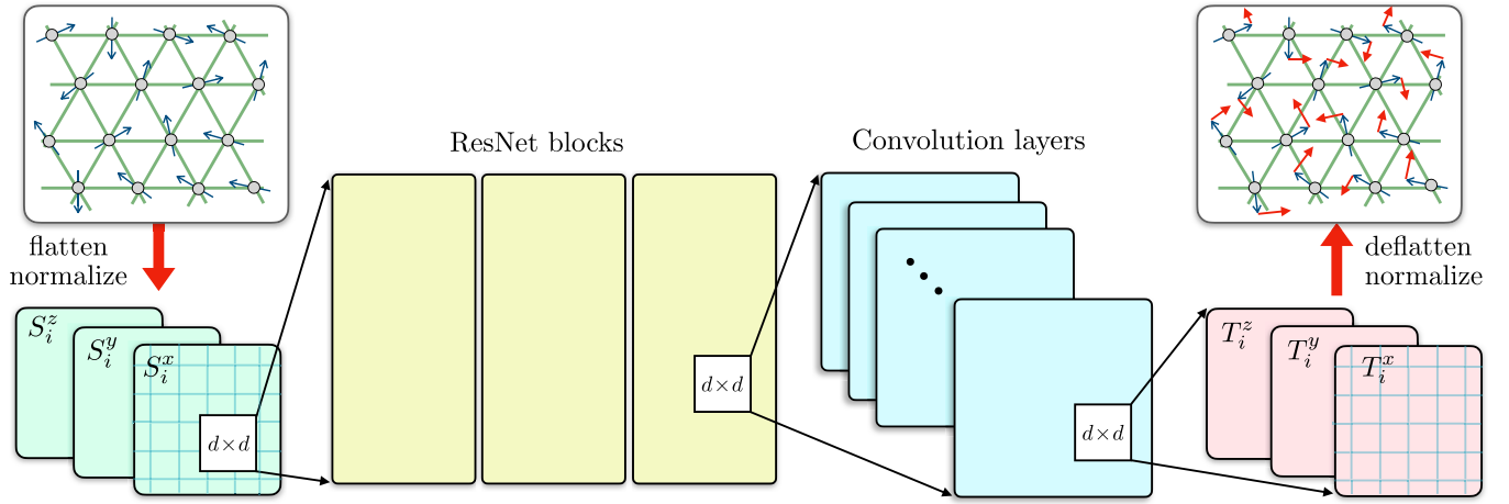
FIG. 1. Schematic diagram of the CNN-based ML model for spin-torque prediction of itinerant electron magnets. The spin configuration \{S_i\} on a lattice is first flattened to give three arrays, corresponding to the three components of spins, which are input to a series of ResNet blocks. Details of the ResNet are presented in Fig. 2. The output of the ResNet blocks is then processed through additional convolution layers. The final output are three arrays which after deflating correspond to the torques \{T_i\} that drive the spin dynamics.
