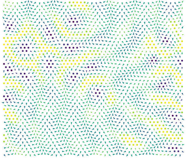
FIG. 6. Snapshot of the spin configuration at the end of the LLG simulation with random initial conditions on a 48 \times 48 triangular lattice.
