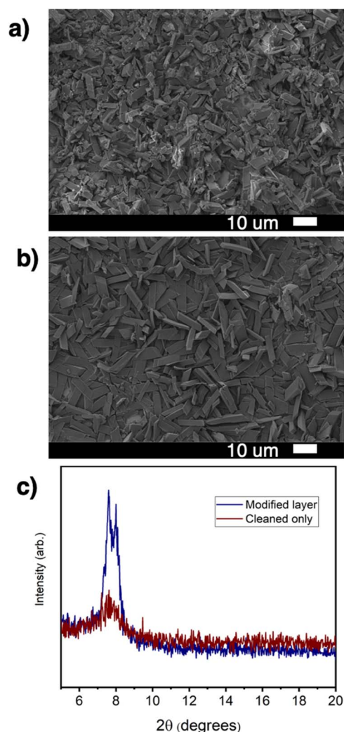
Fig. 4 (a) Co-III ppg cage allowed to crystallize out of DMF on a cleaned, unmodified gold surface. (b) Co-III ppg cage allowed to crystallize out of DMF on an azide-modified gold surface that was first subjected to click reaction with Co-III ppg cage. Crystallization conditions were identical between (a) & (b). (c) PXRD of both surfaces.
