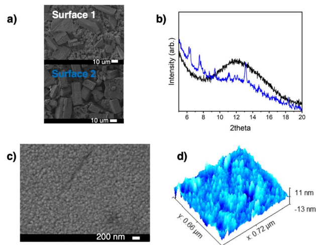
Fig. 3 (a) SEM image of surface 1 where HKUST-1 was solvothermally grown on a gold surface that was modified with an azide followed by click reaction with propargyl amine, & surface 2 where HKUST-1 particles were allowed to deposit on a gold surface that was modified with an azide followed by click reaction with propargyl amine. (b) GIXRD patterns of the surfaces from (a) with the black trace corresponding to surface 1 & the blue trace corresponding to surface 2. (c) SEM image of thin film of HKUST-1 formed from azide modified gold surface after click reaction with propargyl amine-modified HKUST-1 particles. (d) AFM map of surface from (c).
