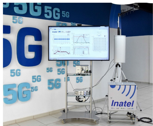
Fig. 15. Prototype of the 5G-RANGE BS.
