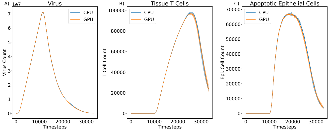
Figure 5: Comparison of aggregate statistics between SIMCoV-CPU (blue) and SIMCoV-GPU (orange) as time-series over the course of a simulated infection. The shaded region shows the minimum and maximum of the statistics across five trials. Plotted are (A) the total count of virus in the simulation, (B) the total count of T cells within the tissue, and (C) the total count of apoptotic epithelial cells.
