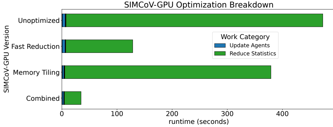
Figure 4: A breakdown of the runtime needed for components of a SIMCoV-GPU simulation broken down by the category of the work being done. Four SIMCoV-GPU versions are plotted: an unoptimized version, a version that only implements fast reductions with shared memory, a version that only implements memory tiling, and finally a version that implements both optimizations.
