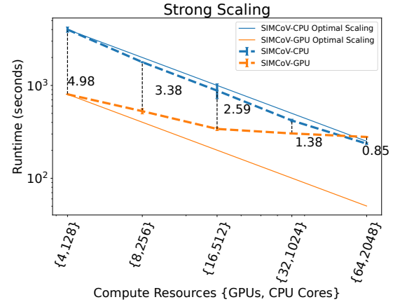
Figure 6: Strong scaling performance of SIMCoV-GPU (orange) versus SIMCoV-CPU (blue). We doubled the number of computational units for each subsequent experiment while maintaining the simulation size throughout. The number of GPUs and CPUs is shown as a tuple in brackets on the x-axis. The runtime of the simulations is plotted on the y-axis in seconds. The plot is on a log-log scale. The speedup of SIMCoV-GPU over SIMCoV-CPU is shown adjacent to the black dashed-line separating the CPU runs and GPU runs. Optimal scaling is approximated by starting with the mean runtime of the smallest scale experiment, and halving it each subsequent experiment.
