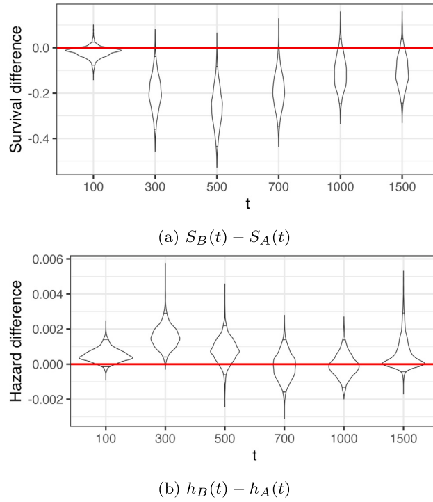
Fig. 8. Small cell lung cancer data. Panels (a) and (b) show, through violin plots, the posterior distributions of the difference between the two treatment survival and hazard functions at six specific time points, t = 100, 300, 500, 700, 1000 , and 1500 days. The short black solid lines within each violin plot indicate the 95% posterior credible interval.
