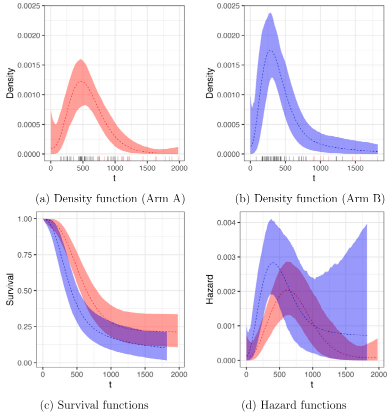
Fig. 7. Small cell lung cancer data. Panels (a) and (b) plot estimates for the Arm A and Arm B density; the rug plots show observed (black) and censored (red) survival times. Panels (c) and (d) compare the estimates for the survival and hazard function. In each panel, the dashed lines denote the posterior mean estimates, and the shaded regions indicate the 95% credible intervals. Red and blue color is used for the Arm A and Arm B group, respectively.
