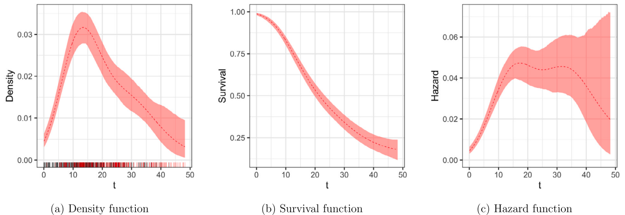
Fig. 6. Liver metastases data. Panels (a), (b) and (c) plot posterior mean (dashed lines) and 95% interval estimates (shaded regions) for the density, survival and hazard function, respectively. The rug plot in panel (a) shows observed (black) and censored (red) survival times.
