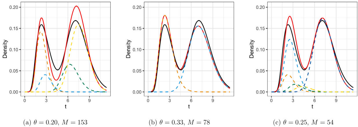
Fig. 3. Simulation Example 1. Plots (a)–(c) show the posterior realization of f(t | M, \theta, G) (red solid line), based on three randomly chosen posterior samples. Each dashed line represents the Erlang basis density \text{Er}(t | m, \theta) for components with \omega_m > 0.01 , multiplied by its corresponding weight. The black solid line is the true underlying density.
