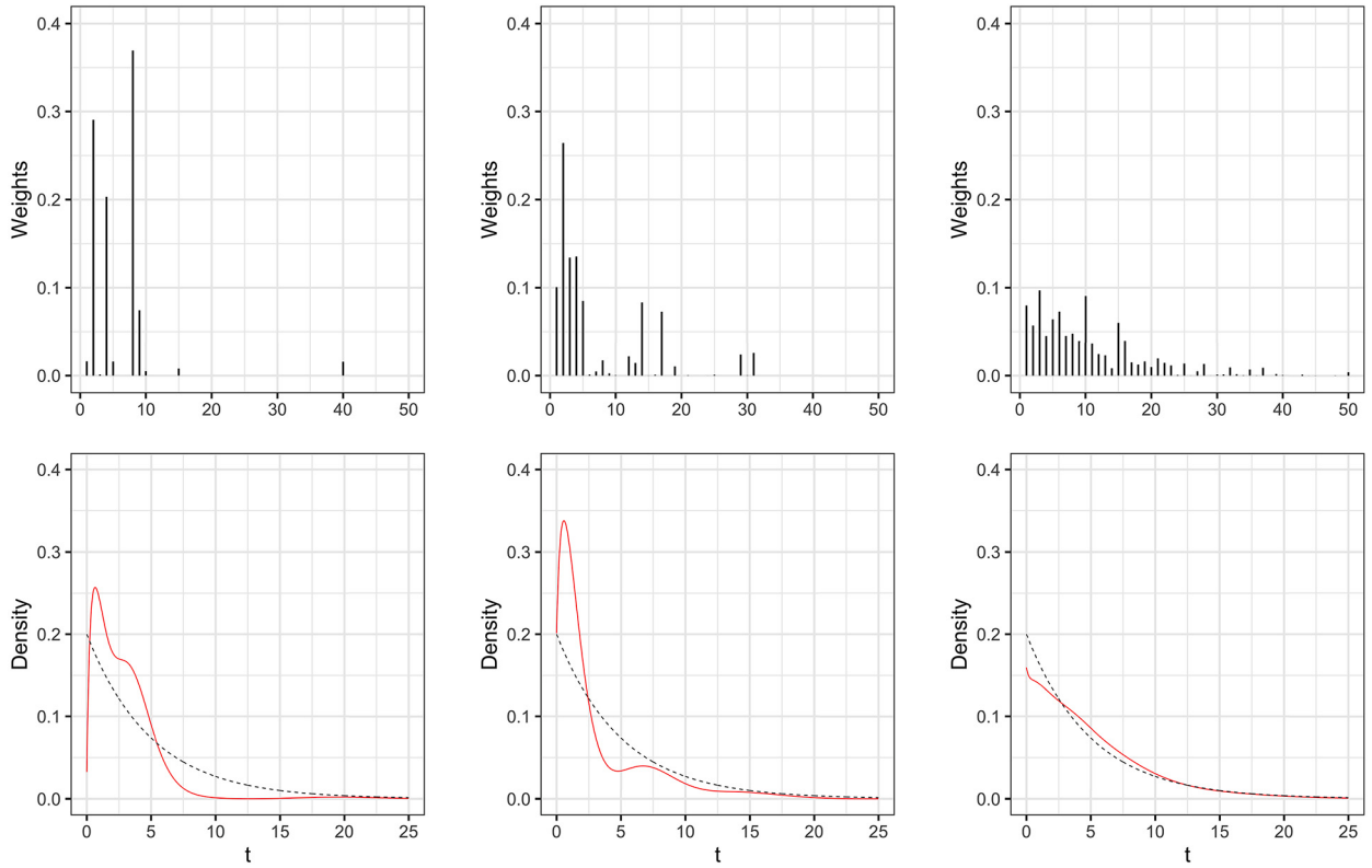
Fig. 1. Prior realizations of the mixture weights \omega (top row) and the corresponding densities f(t | M, \theta, G) given by the red solid lines (bottom row), under \alpha = 1, 10, 100 (left, middle, right columns). In all cases, M = 50 , \theta = 0.5 , and G_0 = \text{Exp}(5) . The black dotted line in the bottom row panels is the density of G_0 . (For interpretation of the colors in the figure(s), the reader is referred to the web version of this article.)
