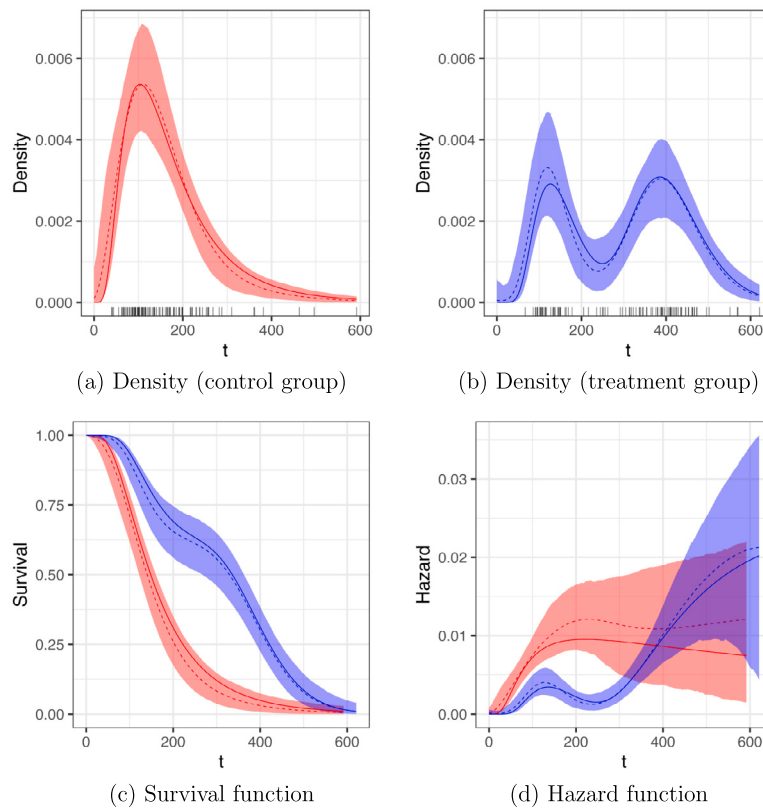
Fig. 5. Simulation Example 3. Panels (a) and (b) plot the estimates for the control and treatment group density, respectively (the rug plots show the corresponding survival times). Panels (c) and (d) compare the estimates for the survival and hazard function, respectively. In each panel, the dashed lines denote the posterior mean estimates, the solid line the true underlying function, and the shaded regions indicate the 95% credible intervals. Red and blue color is used for the control and treatment group, respectively.
