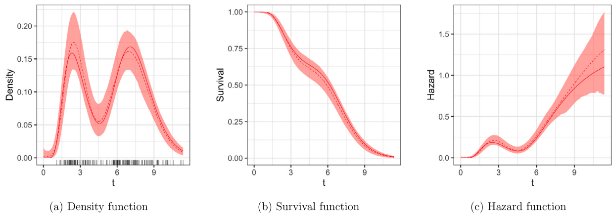
Fig. 2. Simulation Example 1. Posterior mean (dashed lines) and 95% interval estimates (shaded regions) for the density function (left panel), survival function (middle panel) and hazard function (right panel). The red solid line in each panel corresponds to the true underlying function. The black marks on the x-axis in the left panel show the observed survival times.
