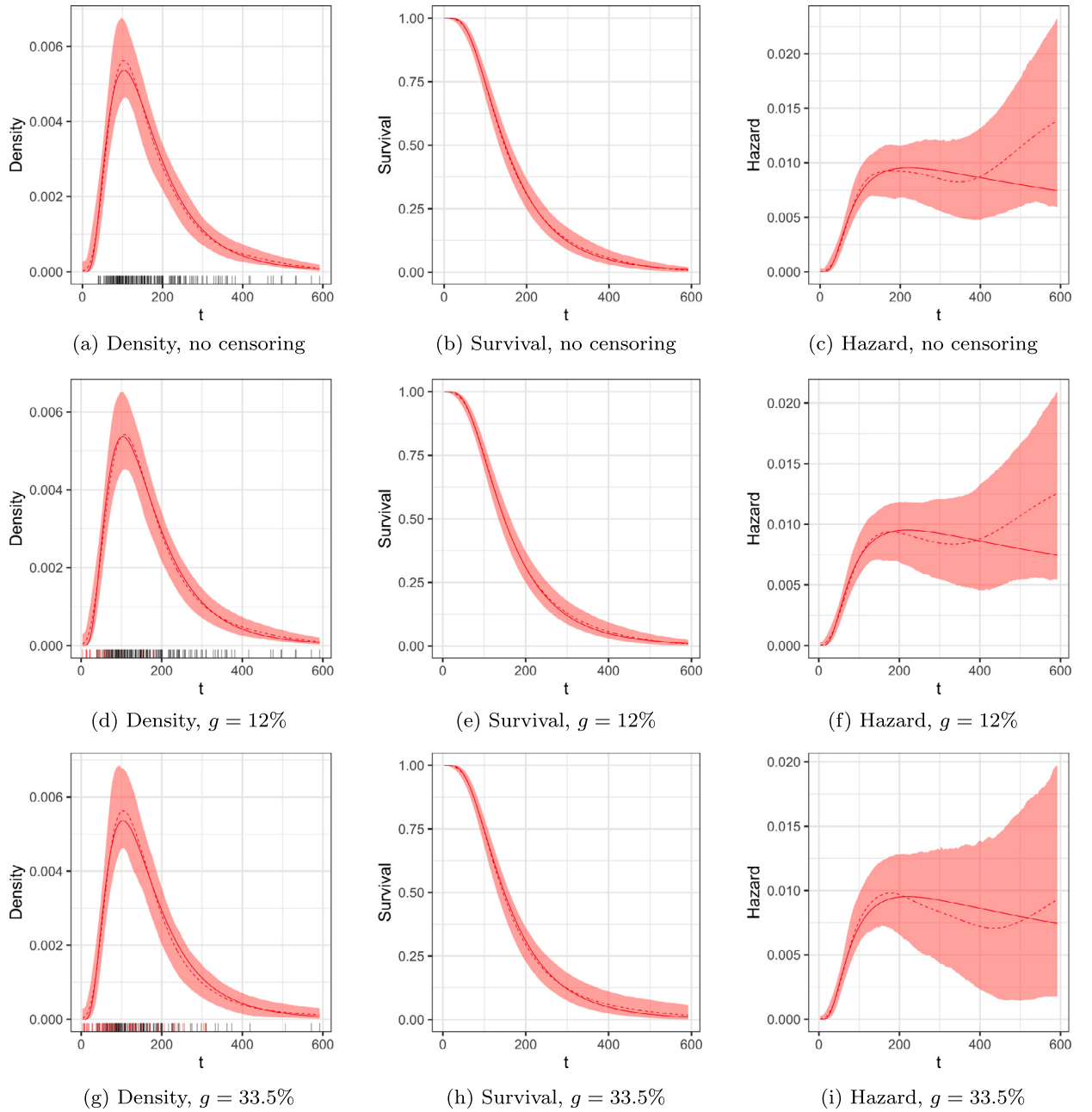
Fig. 4. Simulation Example 2. Posterior mean (dashed lines) and 95% interval estimates (shaded regions) for the density function (left panel), survival function (middle panel) and hazard function (right panel). The red solid line in each panel corresponds to the true underlying function, and the black and red rugs in the left panel show the survival and censoring times, respectively. For the results in the first row, the survival times are fully observed, whereas 12% and 33.5% of the observations are censored for those in the second and third rows, respectively.
