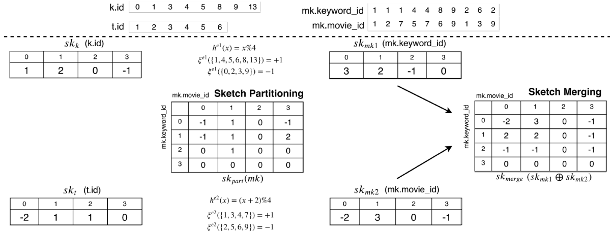
Figure 4: Fast-AGMS sketches for multi-way join cardinality estimation on query JOB 6a.
