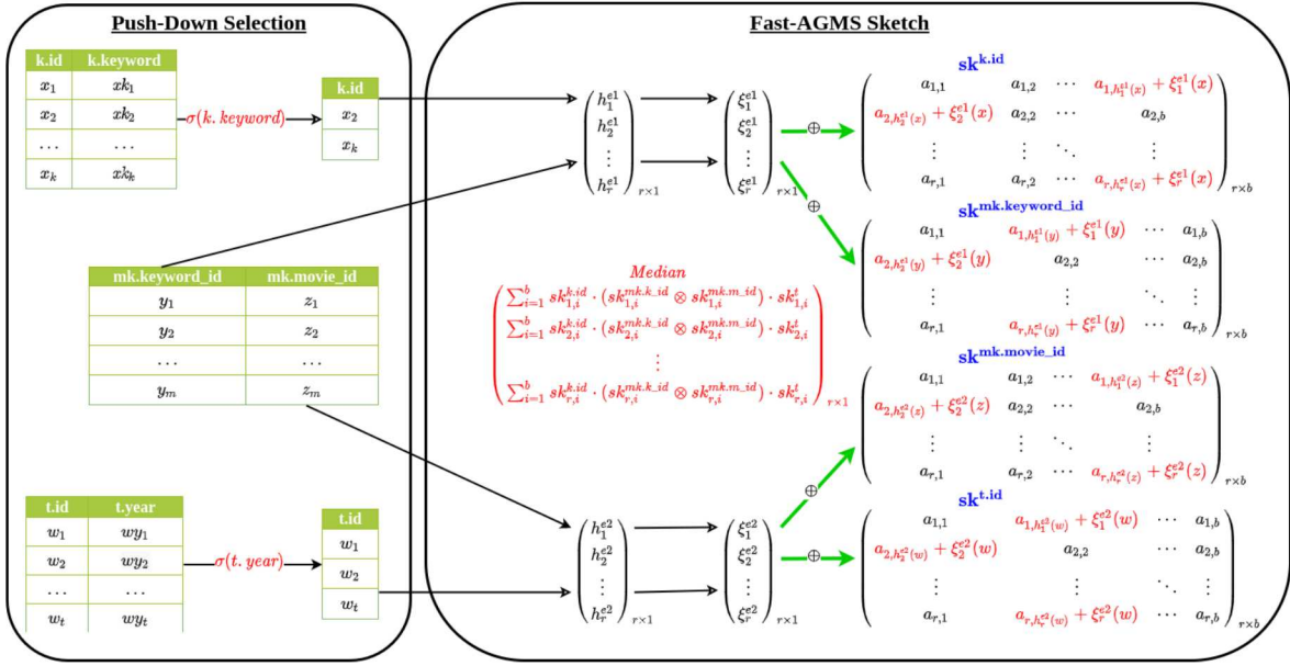
Figure 3: Cardinality estimation for query JOB 6a with (Fast-)AGMS sketches.
