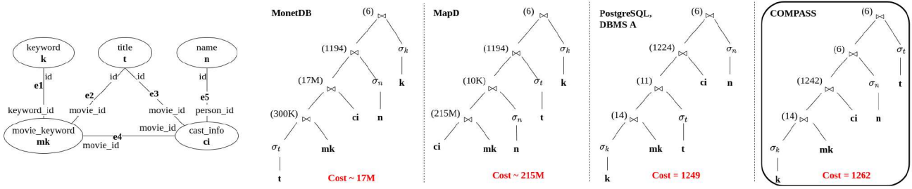
Figure 1: Join graph and corresponding execution plans for query JOB 6a. The numbers represent cardinality.
