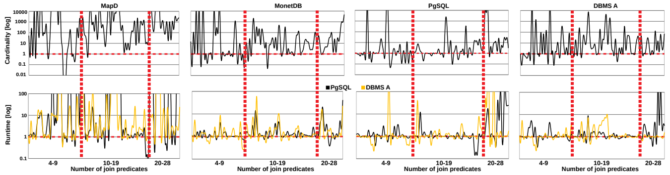
Figure 6: Cardinality and runtime – in PostgreSQL and DBMS A – as a normalized ratio to COMPASS.
