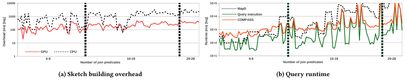
Figure 8: Performance of the COMPASS optimizer implementation in MapD.
