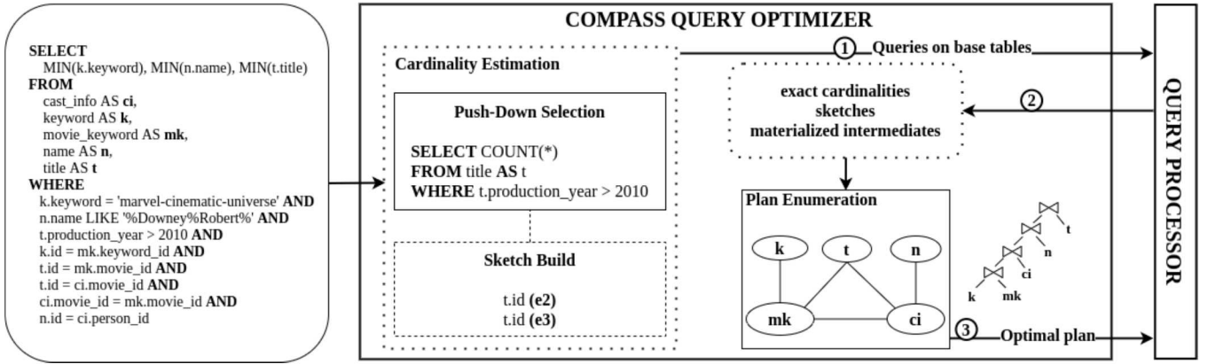
Figure 2: COMPASS workflow: online sketch-based query optimization for in-memory databases.
