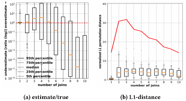
Figure 5: Accuracy ratio (a) and L1-distance between the estimated sketch permutation and the correct join order (b).
