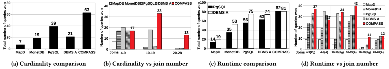
Figure 7: Distribution of winning queries in terms of cardinality and runtime in PostgreSQL and DBMS A.
