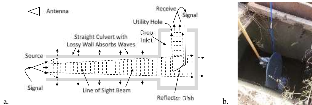
Figure 6. Line of sight wireless telemetry inside of small culvert with challenging drop inlet geometry: a. Geometry, and b. Use of reflector dish antenna in drop inlet, Figure 6.
