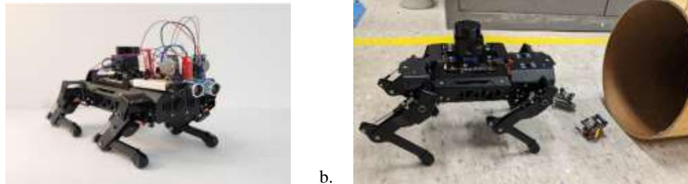
Figure 4 QRDs set up for structural inspection in confined spaces: a. Modified with multi-sensor module, and b. Teamed with microrobots that use vibratory locomotion and FPV cameras.
