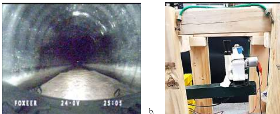
Figure 5 Example sensing options: a. FPV camera view from inside culvert [5], and b. Mechanical tapper with digital microphone for bridge deck sensing undergoing laboratory tests.
