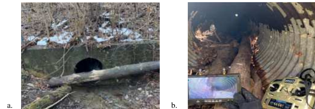
Figure 1 Small culvert with difficult access for humans: a. Exterior entrance, and b. Inside view with other entrance visible [5].
