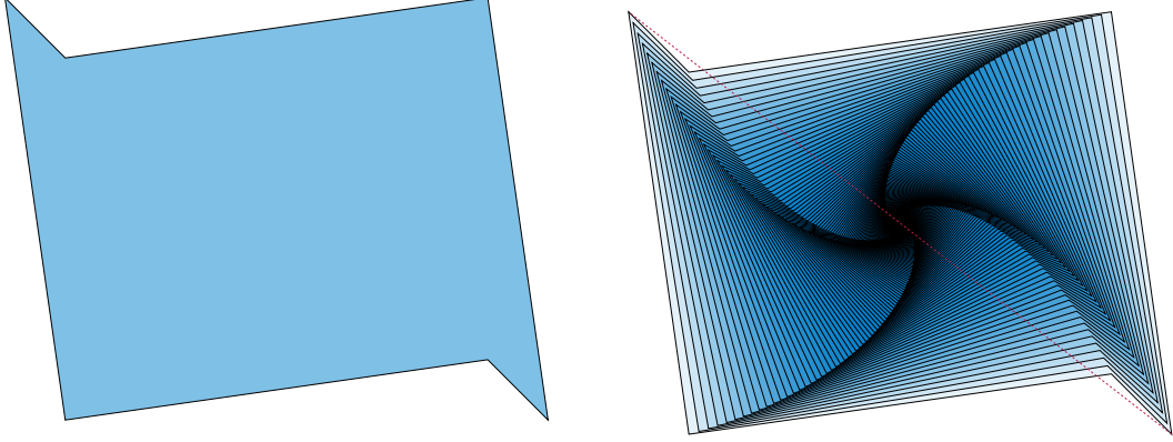
■ Figure 1 A polygon (left) with a continuous shrinking motion (right). The red dashed line connecting two opposite corners through the center of the motion demonstrates that this polygon is not star-shaped: no point on one side of the red dashed line can see into the corner on the other side of the line. As the polygon shrinks, these corners trace out logarithmic spirals; the angle made by these spirals with the red dashed line is the polar tangential angle of its spiral.
